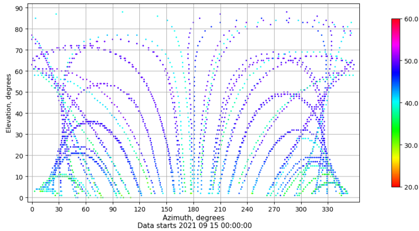
Azimuth-elevation plot for station RIO1. Signal to Noise S1C Data file RIO100ESP_R_2021258.xtr
