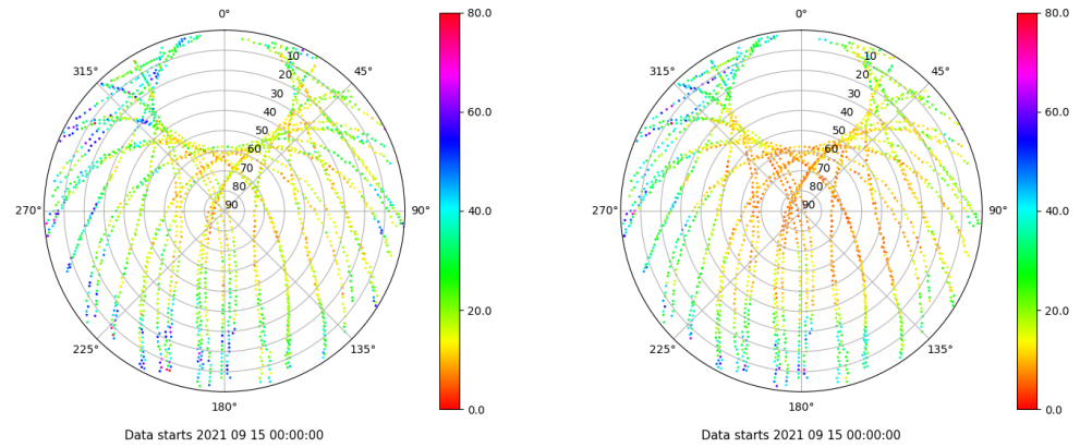
Skyplot for station RIO1. Parameter M1C Data file RIO100ESP_R_2021258.xtr Skyplot for station RIO1. Parameter M2P Data file RIO100ESP_R_2021258.xtr
