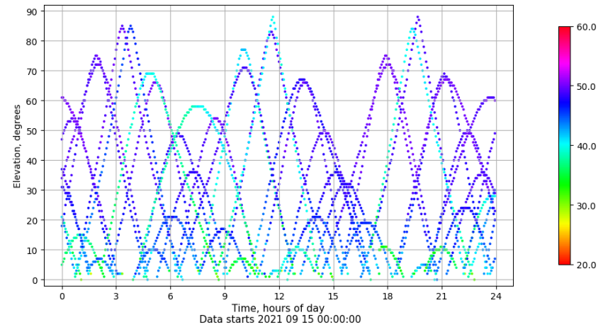
Time-elevation plot for station RIO1. Signal to Noise S1C Data file RIO100ESP_R_2021258.xtr
