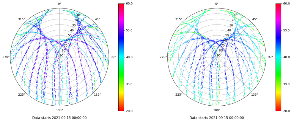
Skyplot for station RIO1. Signal to Noise S1C Data file RIO100ESP_R_2021258.xtr Skyplot for station RIO1. Signal to Noise S2P Data file RIO100ESP_R_2021258.xtr
