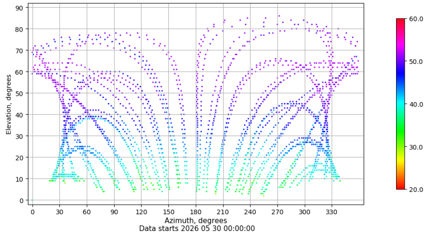
Azimuth-elevation plot for station PUIG. Signal to Noise S1C Data file PUIG00ESP_R_2026150.xtr
