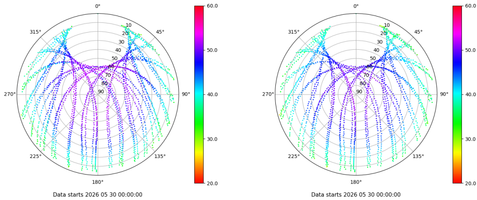
Skyplot for station PUIG. Signal to Noise S1C Data file PUIG00ESP_R_2026150.xtr Skyplot for station PUIG. Signal to Noise S2C Data file PUIG00ESP_R_2026150.xtr
