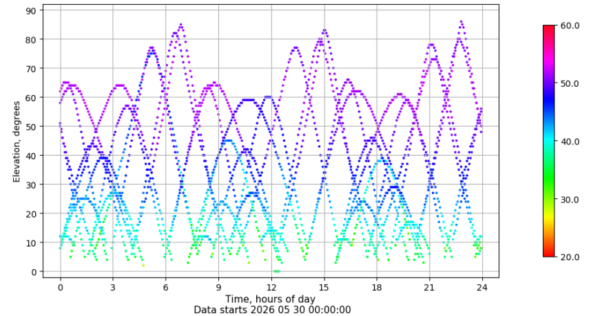
Time-elevation plot for station PUIG. Signal to Noise S1C Data file PUIG00ESP_R_2026150.xtr
