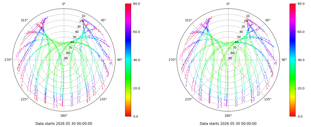
Skyplot for station PUIG. Parameter M1C Data file PUIG00ESP_R_2026150.xtr Skyplot for station PUIG. Parameter M2C Data file PUIG00ESP_R_2026150.xtr
