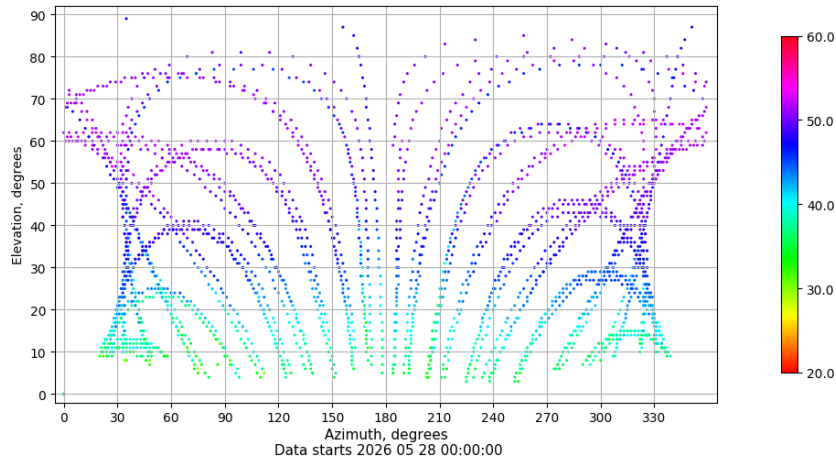
Azimuth-elevation plot for station PUIG. Signal to Noise S1C Data file PUIG00ESP_R_2026148.xtr
