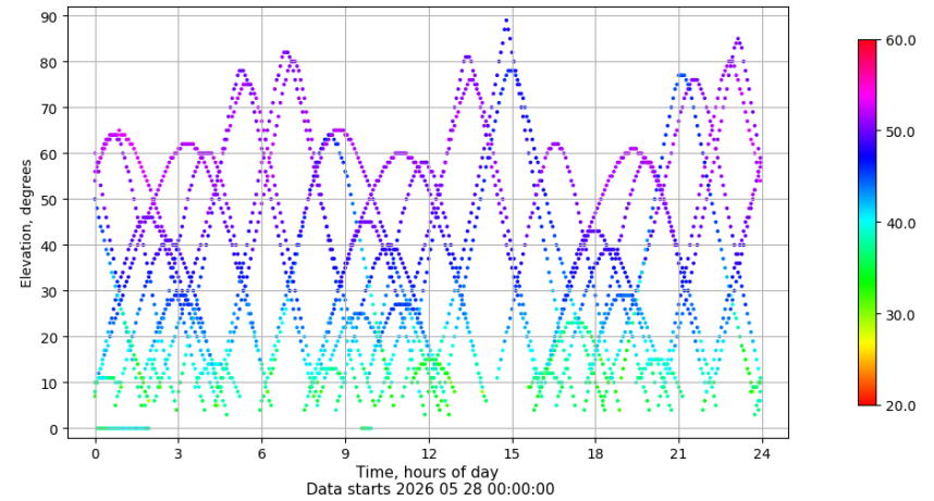
Time-elevation plot for station PUIG. Signal to Noise S1C Data file PUIG00ESP_R_2026148.xtr
