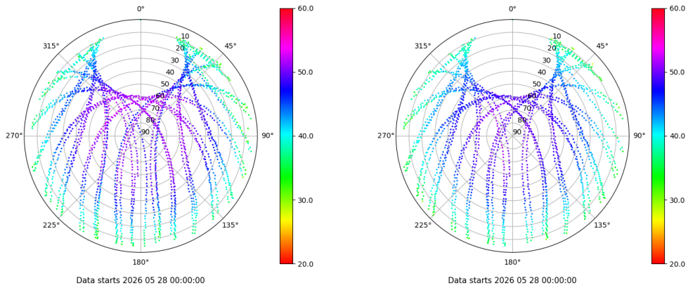
Skyplot for station PUIG. Signal to Noise S1C Data file PUIG00ESP_R_2026148.xtr Skyplot for station PUIG. Signal to Noise S2C Data file PUIG00ESP_R_2026148.xtr
