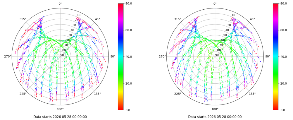
Skyplot for station PUIG. Parameter M1C Data file PUIG00ESP_R_2026148.xtr Skyplot for station PUIG. Parameter M2C Data file PUIG00ESP_R_2026148.xtr
