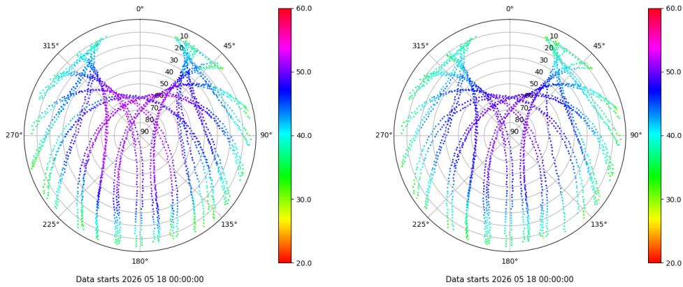
Skyplot for station PUIG. Signal to Noise S1C Data file PUIG00ESP_R_2026138.xtr Skyplot for station PUIG. Signal to Noise S2C Data file PUIG00ESP_R_2026138.xtr
