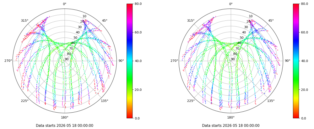
Skyplot for station PUIG. Parameter M1C Data file PUIG00ESP_R_2026138.xtr Skyplot for station PUIG. Parameter M2C Data file PUIG00ESP_R_2026138.xtr
