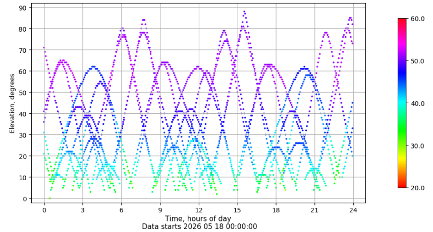
Time-elevation plot for station PUIG. Signal to Noise S1C Data file PUIG00ESP_R_2026138.xtr
