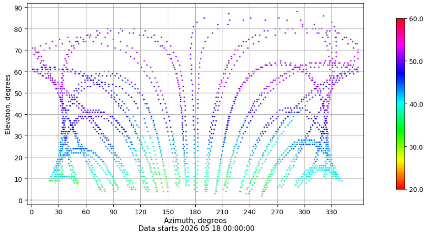
Azimuth-elevation plot for station PUIG. Signal to Noise S1C Data file PUIG00ESP_R_2026138.xtr
