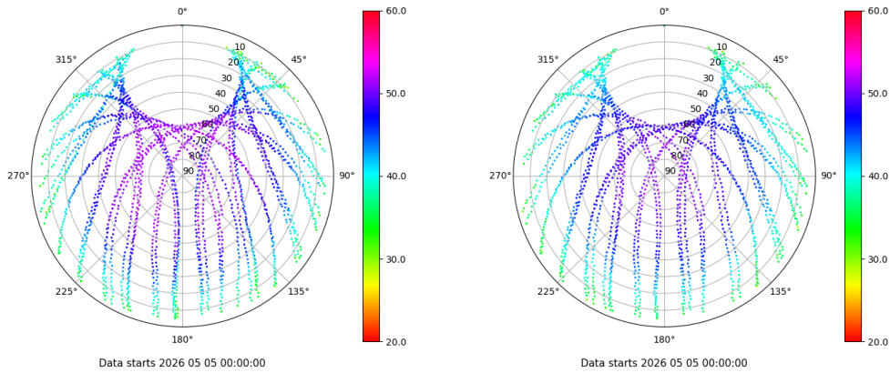
Skyplot for station PUIG. Signal to Noise S1C Data file PUIG00ESP_R_2026125.xtr Skyplot for station PUIG. Signal to Noise S2C Data file PUIG00ESP_R_2026125.xtr
