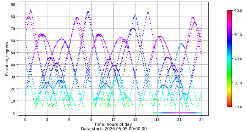
Time-elevation plot for station PUIG. Signal to Noise S1C Data file PUIG00ESP_R_2026125.xtr
