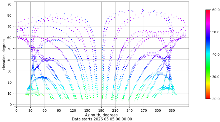
Azimuth-elevation plot for station PUIG. Signal to Noise S1C Data file PUIG00ESP_R_2026125.xtr
