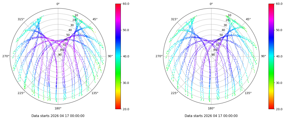
Skyplot for station PUIG. Signal to Noise S1C Data file PUIG00ESP_R_2026107.xtr Skyplot for station PUIG. Signal to Noise S2C Data file PUIG00ESP_R_2026107.xtr
