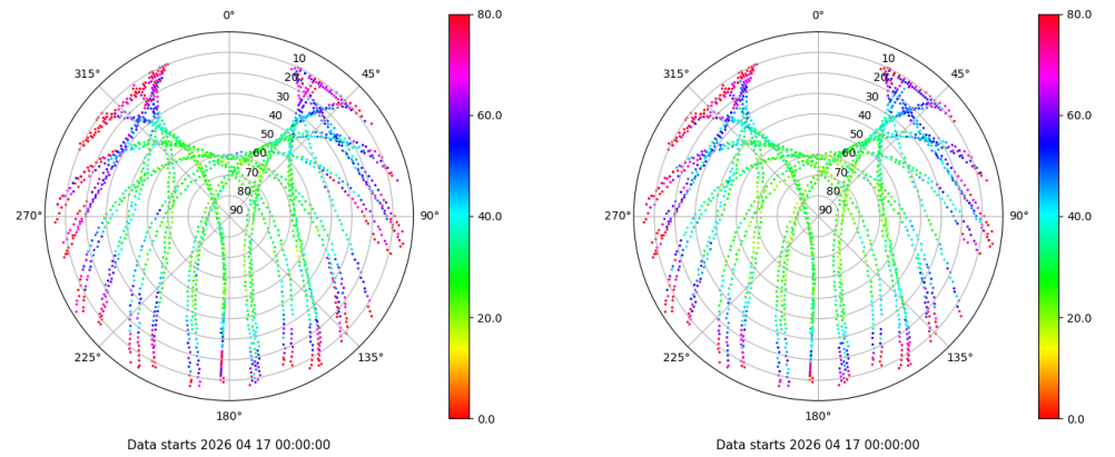
Skyplot for station PUIG. Parameter M1C Data file PUIG00ESP_R_2026107.xtr Skyplot for station PUIG. Parameter M2C Data file PUIG00ESP_R_2026107.xtr
