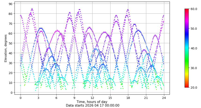
Time-elevation plot for station PUIG. Signal to Noise S1C Data file PUIG00ESP_R_2026107.xtr
