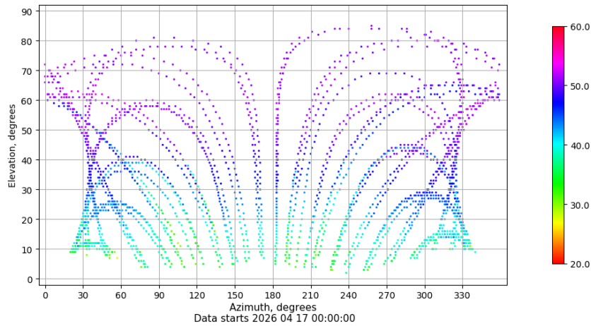
Azimuth-elevation plot for station PUIG. Signal to Noise S1C Data file PUIG00ESP_R_2026107.xtr
