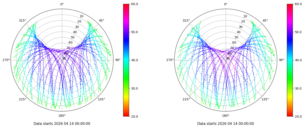
Skyplot for station PUIG. Signal to Noise S1C Data file PUIG00ESP_R_2026104.xtr Skyplot for station PUIG. Signal to Noise S2X Data file PUIG00ESP_R_2026104.xtr
