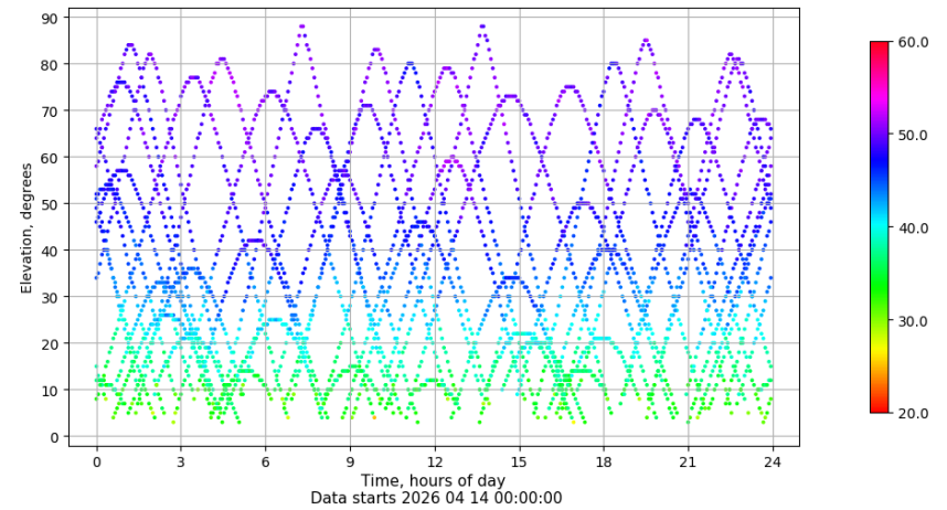
Time-elevation plot for station PUIG. Signal to Noise S1C Data file PUIG00ESP_R_2026104.xtr
