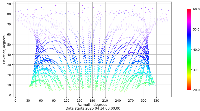
Azimuth-elevation plot for station PUIG. Signal to Noise S1C Data file PUIG00ESP_R_2026104.xtr
