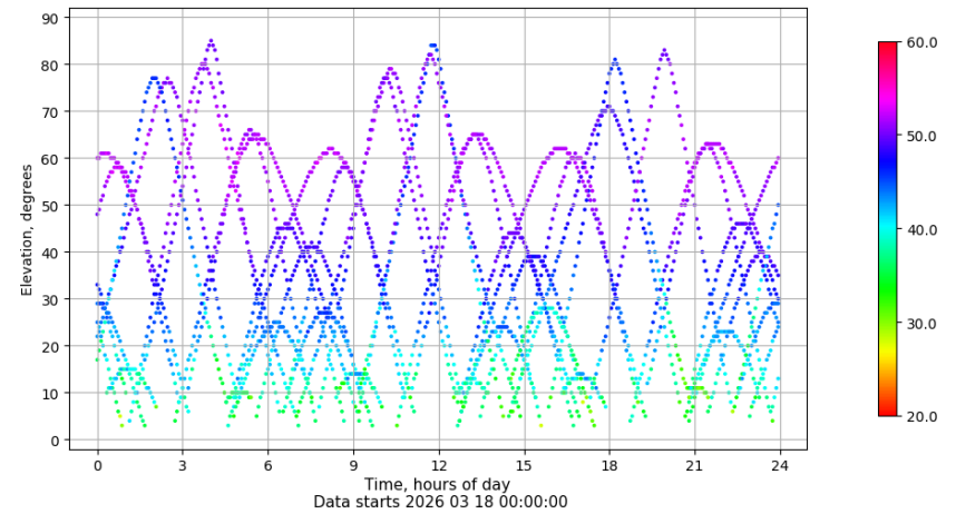
Time-elevation plot for station PUIG. Signal to Noise S1C Data file PUIG00ESP_R_2026077.xtr
