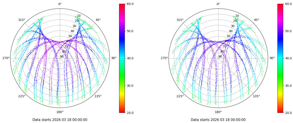
Skyplot for station PUIG. Signal to Noise S1C Data file PUIG00ESP_R_2026077.xtr Skyplot for station PUIG. Signal to Noise S2C Data file PUIG00ESP_R_2026077.xtr
