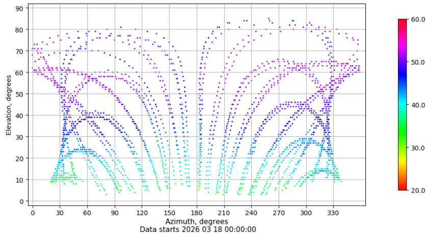
Azimuth-elevation plot for station PUIG. Signal to Noise S1C Data file PUIG00ESP_R_2026077.xtr
