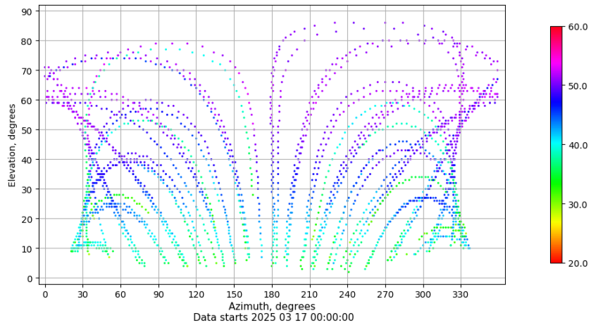
Azimuth-elevation plot for station PUIG. Signal to Noise S1C Data file PUIG00ESP_R_2025076.xtr
