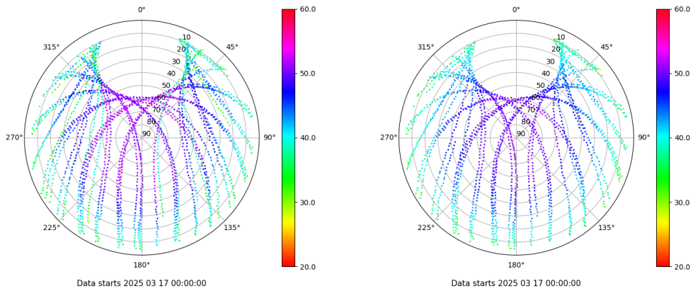
Skyplot for station PUIG. Signal to Noise S1C Data file PUIG00ESP_R_2025076.xtr Skyplot for station PUIG. Signal to Noise S2C Data file PUIG00ESP_R_2025076.xtr
