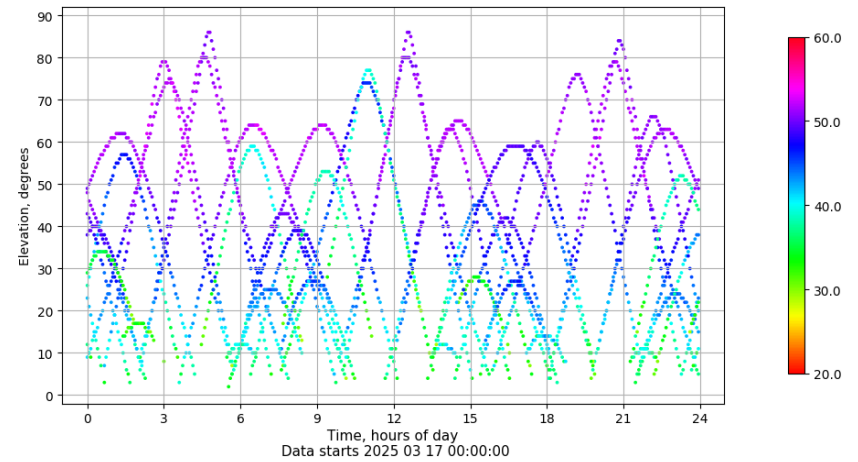
Time-elevation plot for station PUIG. Signal to Noise S1C Data file PUIG00ESP_R_2025076.xtr
