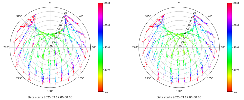
Skyplot for station PUIG. Parameter M1C Data file PUIG00ESP_R_2025076.xtr Skyplot for station PUIG. Parameter M2C Data file PUIG00ESP_R_2025076.xtr
