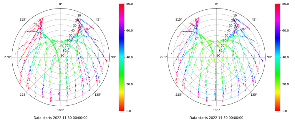
Skyplot for station PUIG. Parameter M1C Data file PUIG00ESP_R_2022334.xtr Skyplot for station PUIG. Parameter M2C Data file PUIG00ESP_R_2022334.xtr
