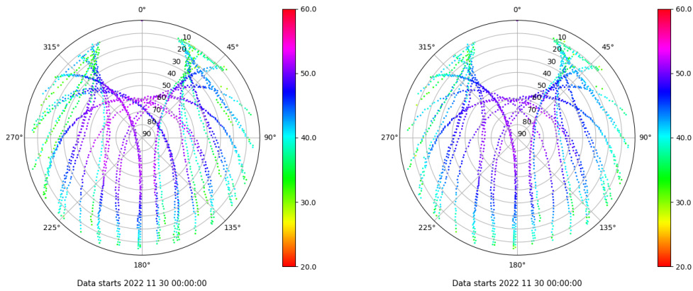
Skyplot for station PUIG. Signal to Noise S1C Data file PUIG00ESP_R_2022334.xtr Skyplot for station PUIG. Signal to Noise S2C Data file PUIG00ESP_R_2022334.xtr
