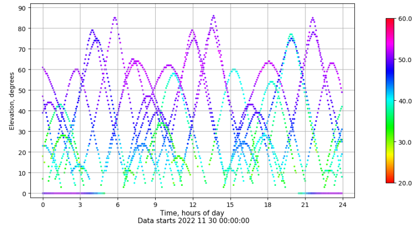
Time-elevation plot for station PUIG. Signal to Noise S1C Data file PUIG00ESP_R_2022334.xtr
