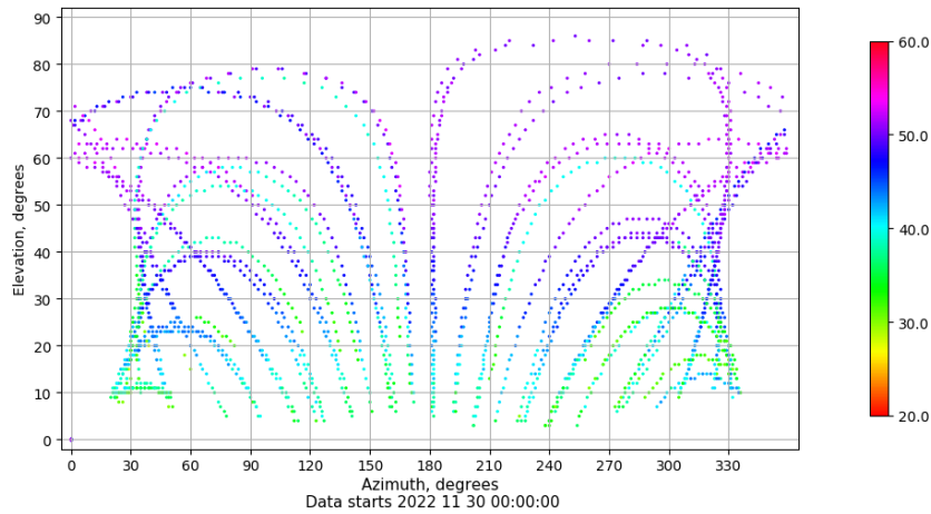
Azimuth-elevation plot for station PUIG. Signal to Noise S1C Data file PUIG00ESP_R_2022334.xtr
