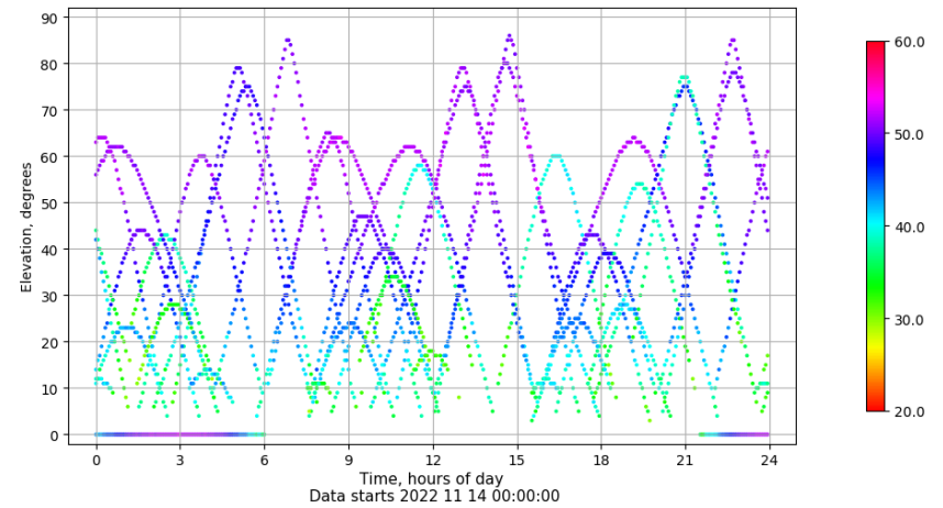
Time-elevation plot for station PUIG. Signal to Noise S1C Data file PUIG00ESP_R_2022318.xtr
