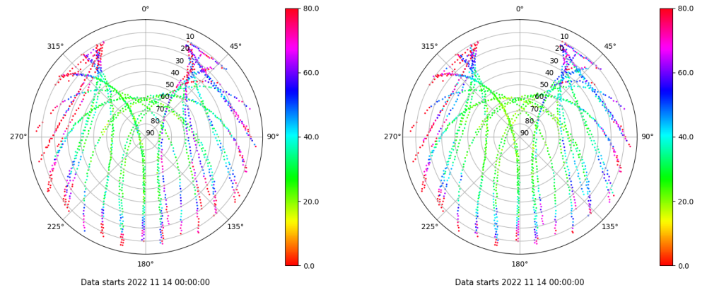
Skyplot for station PUIG. Parameter M1C Data file PUIG00ESP_R_2022318.xtr Skyplot for station PUIG. Parameter M2C Data file PUIG00ESP_R_2022318.xtr
