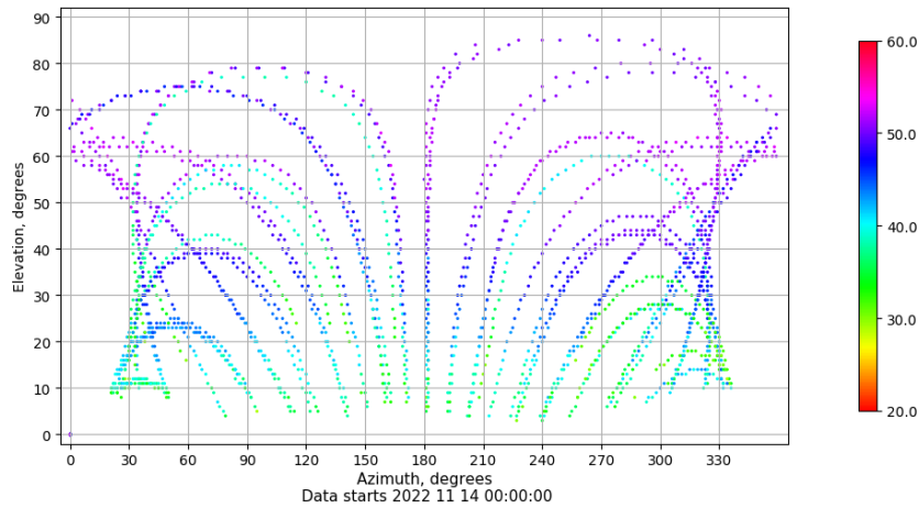
Azimuth-elevation plot for station PUIG. Signal to Noise S1C Data file PUIG00ESP_R_2022318.xtr
