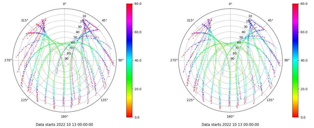
Skyplot for station PUIG. Parameter M1C Data file PUIG00ESP_R_2022286.xtr Skyplot for station PUIG. Parameter M2C Data file PUIG00ESP_R_2022286.xtr
