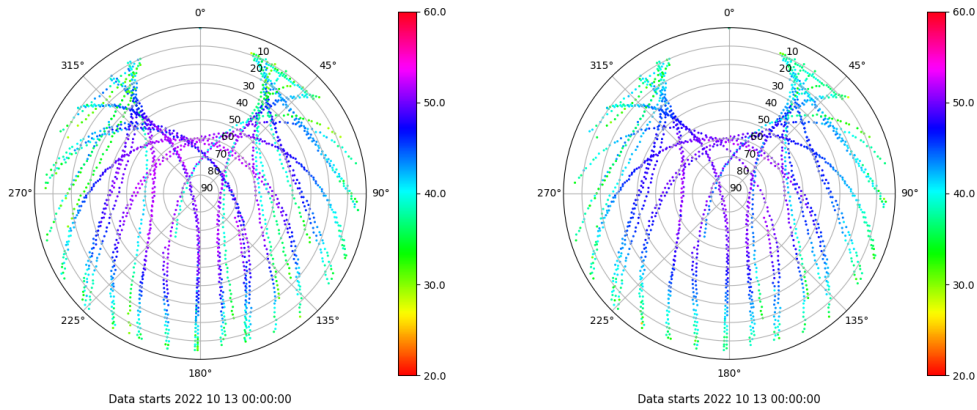
Skyplot for station PUIG. Signal to Noise S1C Data file PUIG00ESP_R_2022286.xtr Skyplot for station PUIG. Signal to Noise S2C Data file PUIG00ESP_R_2022286.xtr
