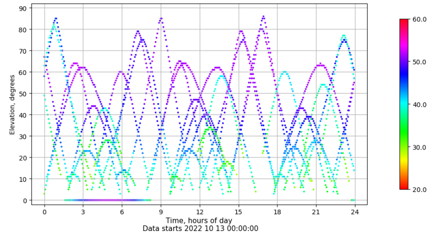
Time-elevation plot for station PUIG. Signal to Noise S1C Data file PUIG00ESP_R_2022286.xtr
