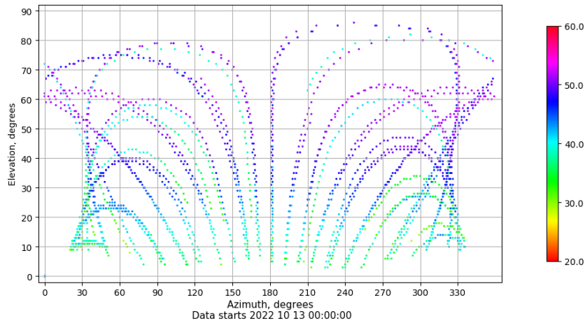
Azimuth-elevation plot for station PUIG. Signal to Noise S1C Data file PUIG00ESP_R_2022286.xtr
