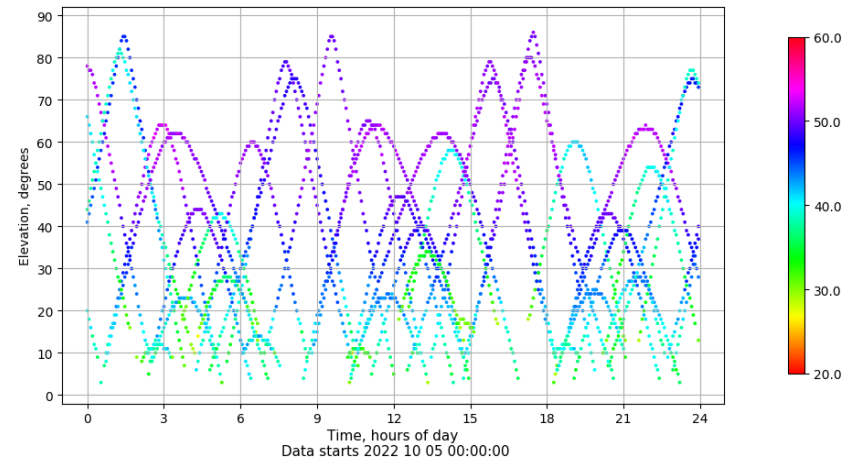
Time-elevation plot for station PUIG. Signal to Noise S1C Data file PUIG00ESP_R_2022278.xtr
