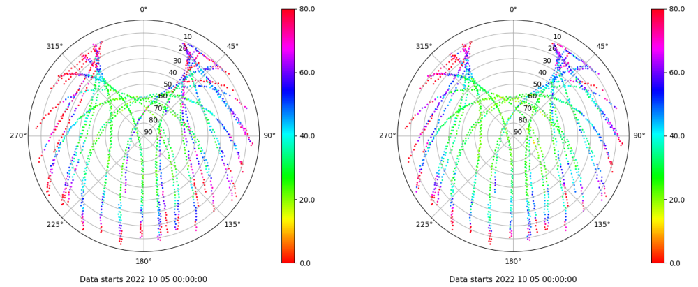
Skyplot for station PUIG. Parameter M1C Data file PUIG00ESP_R_2022278.xtr Skyplot for station PUIG. Parameter M2C Data file PUIG00ESP_R_2022278.xtr
