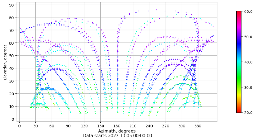
Azimuth-elevation plot for station PUIG. Signal to Noise S1C Data file PUIG00ESP_R_2022278.xtr
