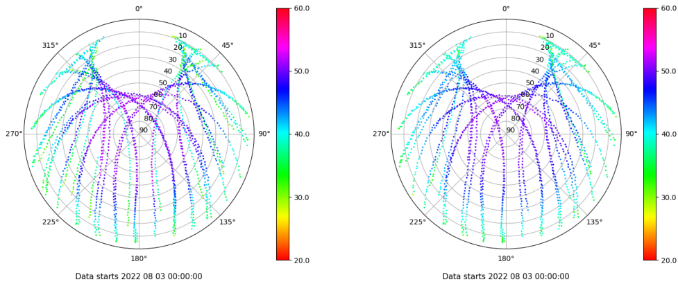
Skyplot for station PUIG. Signal to Noise S1C Data file PUIG00ESP_R_2022215.xtr Skyplot for station PUIG. Signal to Noise S2C Data file PUIG00ESP_R_2022215.xtr
