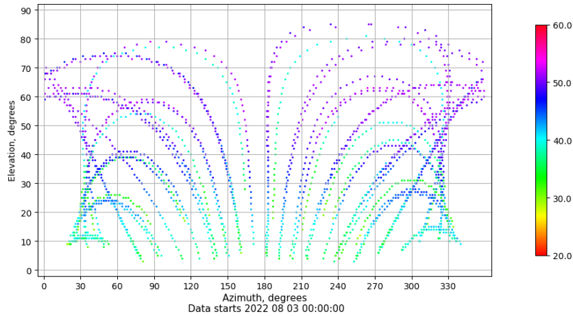
Azimuth-elevation plot for station PUIG. Signal to Noise S1C Data file PUIG00ESP_R_2022215.xtr
