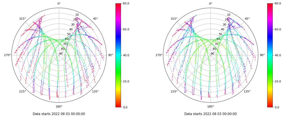
Skyplot for station PUIG. Parameter M1C Data file PUIG00ESP_R_2022215.xtr Skyplot for station PUIG. Parameter M2C Data file PUIG00ESP_R_2022215.xtr
