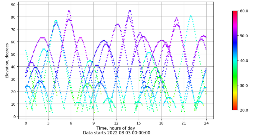
Time-elevation plot for station PUIG. Signal to Noise S1C Data file PUIG00ESP_R_2022215.xtr
