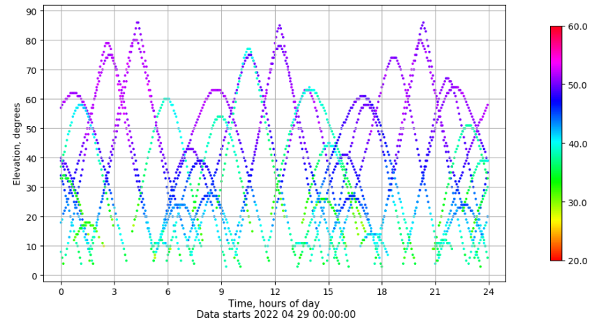
Time-elevation plot for station PUIG. Signal to Noise S1C Data file PUIG00ESP_R_2022119.xtr
