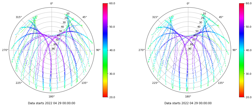
Skyplot for station PUIG. Signal to Noise S1C Data file PUIG00ESP_R_2022119.xtr Skyplot for station PUIG. Signal to Noise S2C Data file PUIG00ESP_R_2022119.xtr
