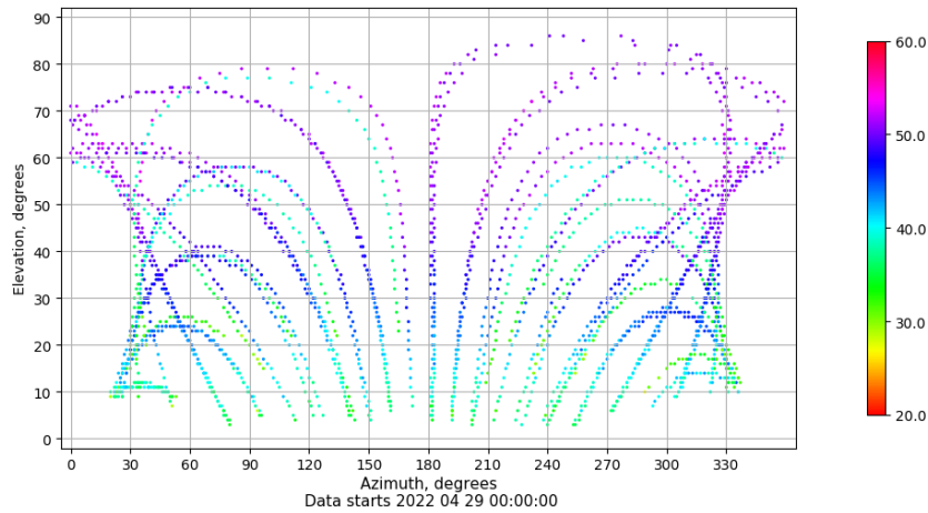
Azimuth-elevation plot for station PUIG. Signal to Noise S1C Data file PUIG00ESP_R_2022119.xtr
