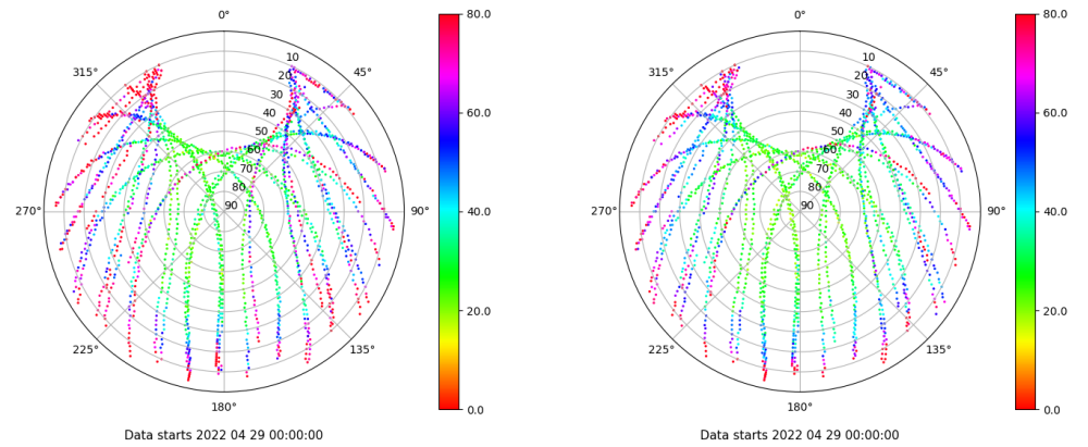
Skyplot for station PUIG. Parameter M1C Data file PUIG00ESP_R_2022119.xtr Skyplot for station PUIG. Parameter M2C Data file PUIG00ESP_R_2022119.xtr
