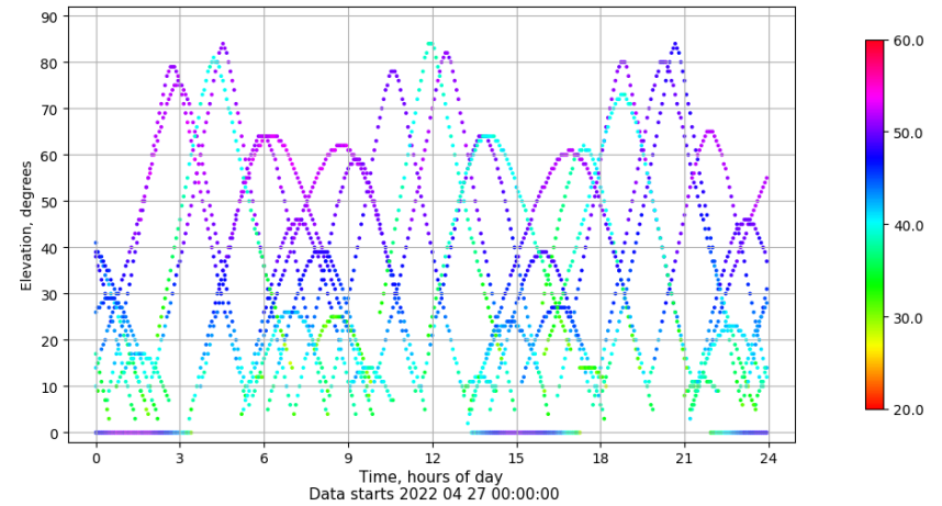
Time-elevation plot for station PUIG. Signal to Noise S1C Data file PUIG00ESP_R_2022117.xtr
