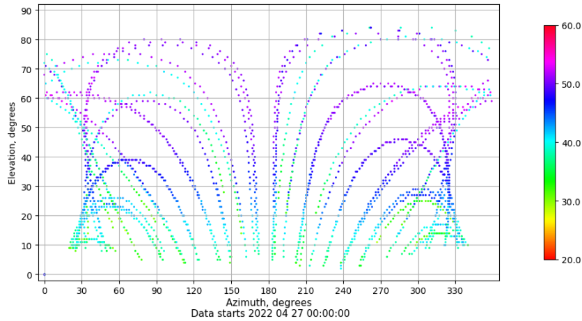
Azimuth-elevation plot for station PUIG. Signal to Noise S1C Data file PUIG00ESP_R_2022117.xtr
