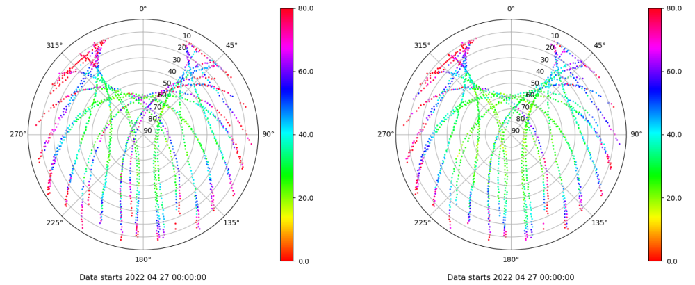
Skyplot for station PUIG. Parameter M1C Data file PUIG00ESP_R_2022117.xtr Skyplot for station PUIG. Parameter M2C Data file PUIG00ESP_R_2022117.xtr
