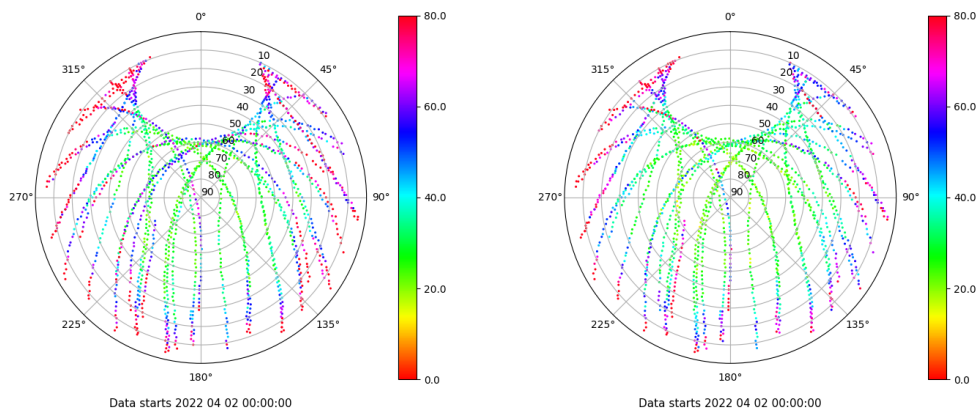
Skyplot for station PUIG. Parameter M1C Data file PUIG00ESP_R_2022092.xtr Skyplot for station PUIG. Parameter M2C Data file PUIG00ESP_R_2022092.xtr
