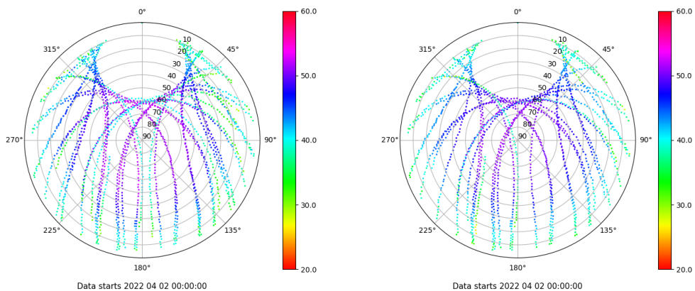
Skyplot for station PUIG. Signal to Noise S1C Data file PUIG00ESP_R_2022092.xtr Skyplot for station PUIG. Signal to Noise S2C Data file PUIG00ESP_R_2022092.xtr
