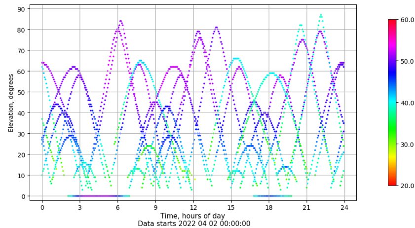
Time-elevation plot for station PUIG. Signal to Noise S1C Data file PUIG00ESP_R_2022092.xtr
