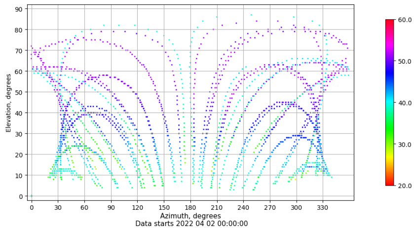
Azimuth-elevation plot for station PUIG. Signal to Noise S1C Data file PUIG00ESP_R_2022092.xtr
