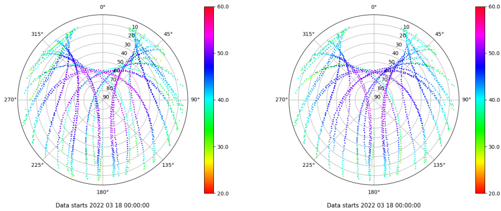
Skyplot for station PUIG. Signal to Noise S1C Data file PUIG00ESP_R_2022077.xtr Skyplot for station PUIG. Signal to Noise S2C Data file PUIG00ESP_R_2022077.xtr
