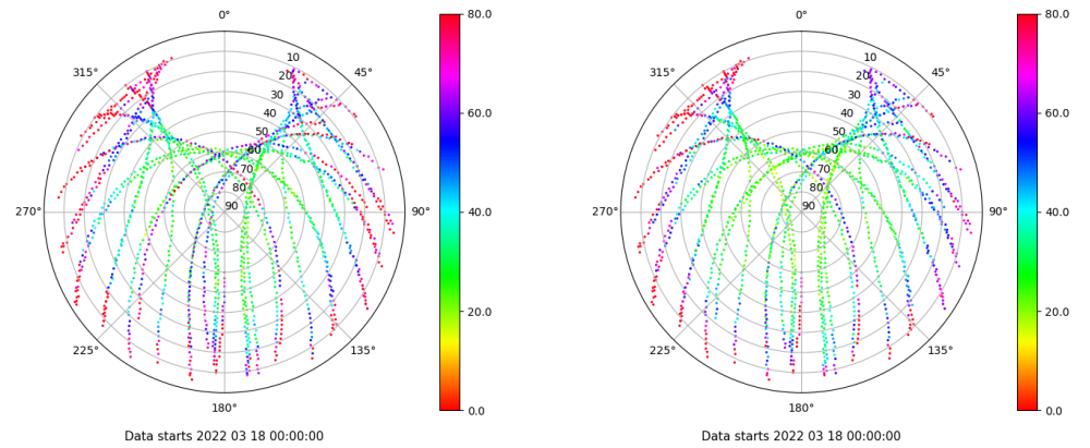
Skyplot for station PUIG. Parameter M1C Data file PUIG00ESP_R_2022077.xtr Skyplot for station PUIG. Parameter M2C Data file PUIG00ESP_R_2022077.xtr
