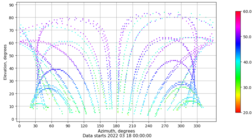
Azimuth-elevation plot for station PUIG. Signal to Noise S1C Data file PUIG00ESP_R_2022077.xtr
