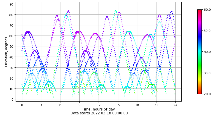
Time-elevation plot for station PUIG. Signal to Noise S1C Data file PUIG00ESP_R_2022077.xtr
