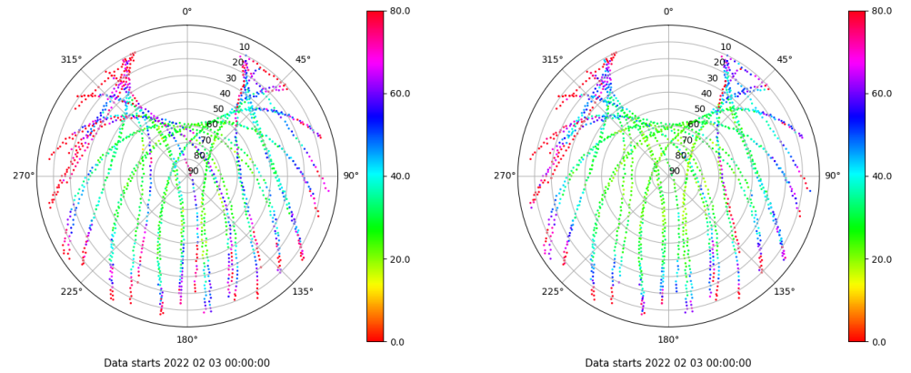
Skyplot for station PUIG. Parameter M1C Data file PUIG00ESP_R_2022034.xtr Skyplot for station PUIG. Parameter M2C Data file PUIG00ESP_R_2022034.xtr
