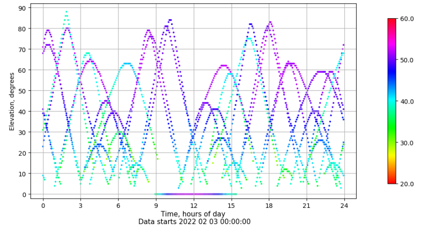
Time-elevation plot for station PUIG. Signal to Noise S1C Data file PUIG00ESP_R_2022034.xtr
