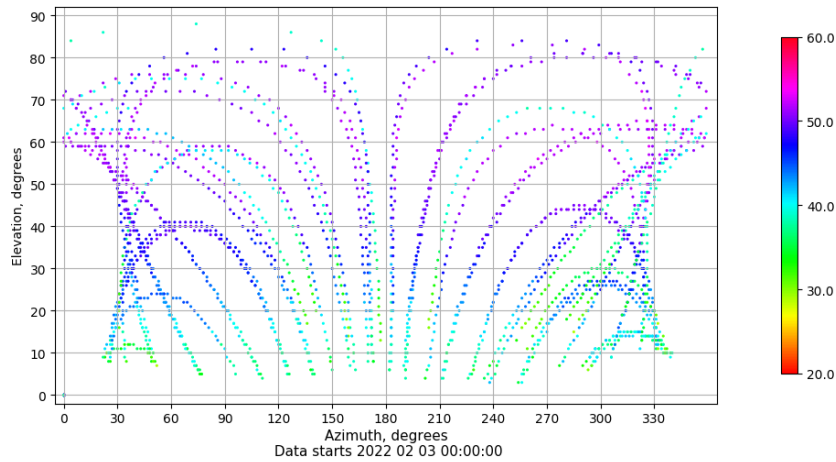
Azimuth-elevation plot for station PUIG. Signal to Noise S1C Data file PUIG00ESP_R_2022034.xtr
