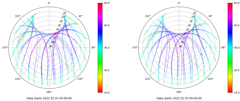
Skyplot for station PUIG. Signal to Noise S1C Data file PUIG00ESP_R_2022034.xtr Skyplot for station PUIG. Signal to Noise S2C Data file PUIG00ESP_R_2022034.xtr
