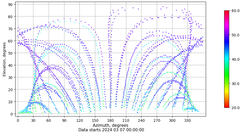
Azimuth-elevation plot for station PENI. Signal to Noise S1C Data file PENI00ESP_R_2024067.xtr
