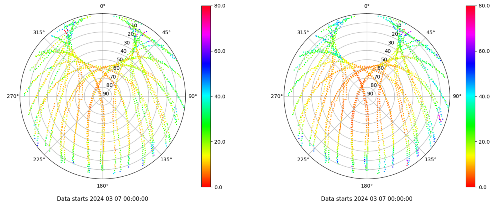
Skyplot for station PENI. Parameter M1C Data file PENI00ESP_R_2024067.xtr Skyplot for station PENI. Parameter M2P Data file PENI00ESP_R_2024067.xtr
