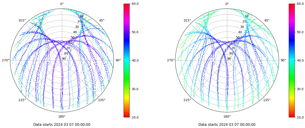
Skyplot for station PENI. Signal to Noise S1C Data file PENI00ESP_R_2024067.xtr Skyplot for station PENI. Signal to Noise S2P Data file PENI00ESP_R_2024067.xtr
