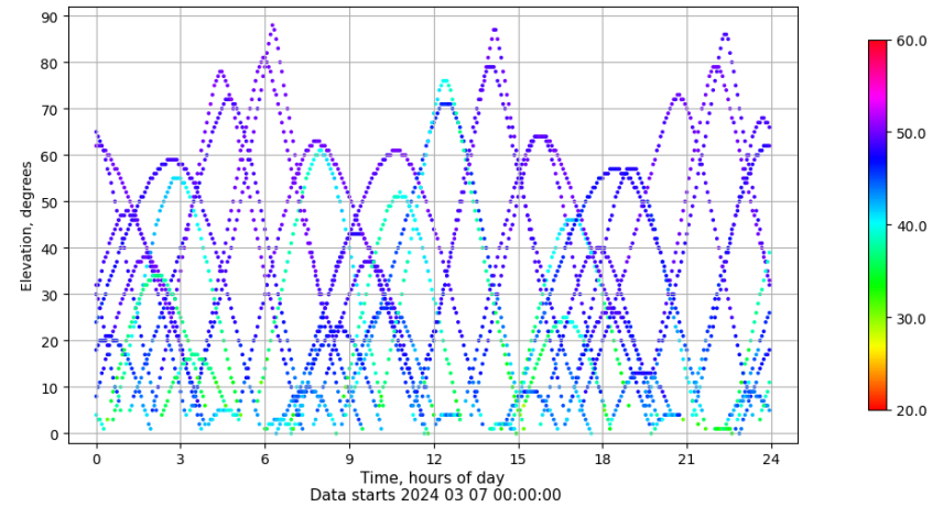
Time-elevation plot for station PENI. Signal to Noise S1C Data file PENI00ESP_R_2024067.xtr
