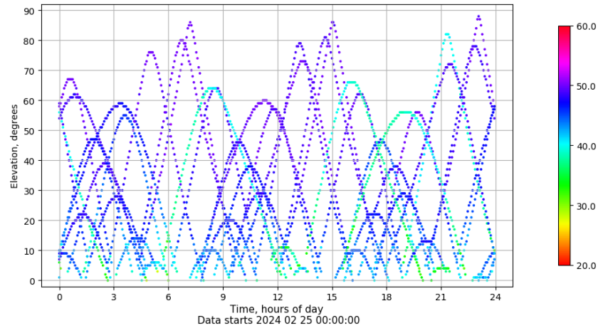
Time-elevation plot for station PENI. Signal to Noise S1C Data file PENI00ESP_R_2024056.xtr
