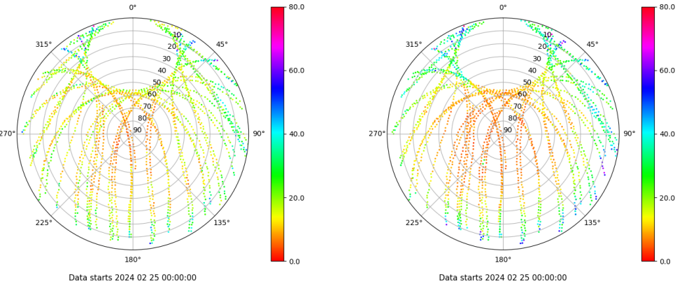
Skyplot for station PENI. Parameter M1C Data file PENI00ESP_R_2024056.xtr Skyplot for station PENI. Parameter M2P Data file PENI00ESP_R_2024056.xtr
