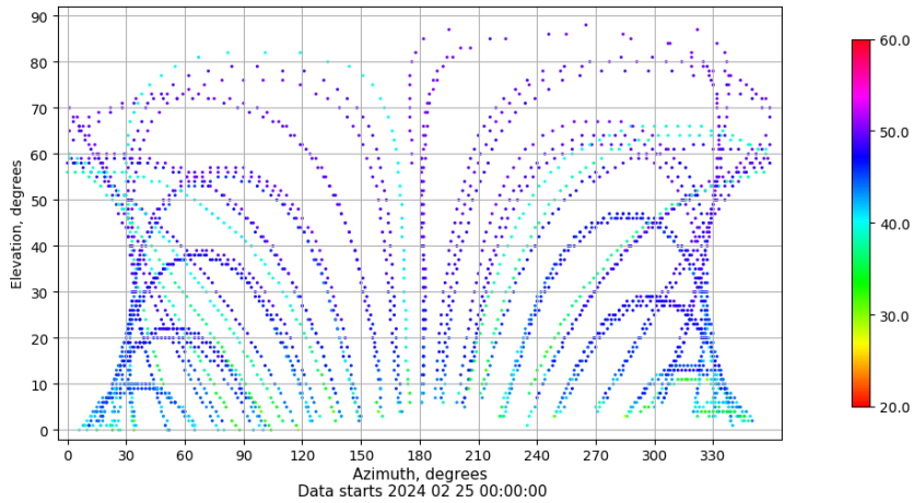
Azimuth-elevation plot for station PENI. Signal to Noise S1C Data file PENI00ESP_R_2024056.xtr
