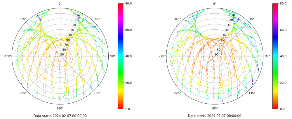
Skyplot for station PENI. Parameter M1C Data file PENI00ESP_R_2024038.xtr Skyplot for station PENI. Parameter M2P Data file PENI00ESP_R_2024038.xtr
