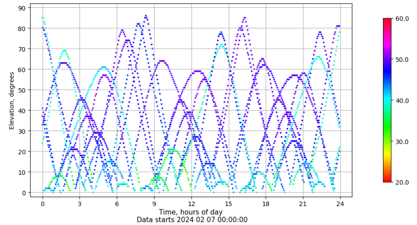
Time-elevation plot for station PENI. Signal to Noise S1C Data file PENI00ESP_R_2024038.xtr
