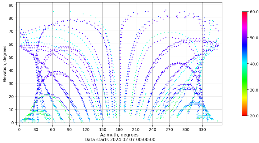
Azimuth-elevation plot for station PENI. Signal to Noise S1C Data file PENI00ESP_R_2024038.xtr
