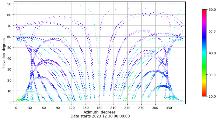
Azimuth-elevation plot for station PENI. Signal to Noise S1C Data file PENI00ESP_R_2023364.xtr
