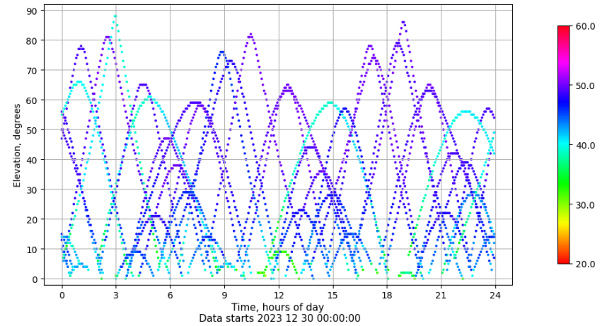
Time-elevation plot for station PENI. Signal to Noise S1C Data file PENI00ESP_R_2023364.xtr
