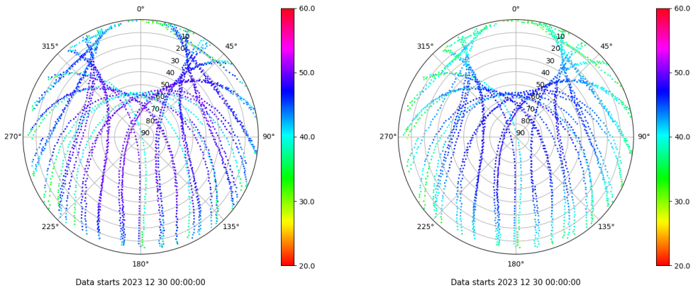
Skyplot for station PENI. Signal to Noise S1C Data file PENI00ESP_R_2023364.xtr Skyplot for station PENI. Signal to Noise S2P Data file PENI00ESP_R_2023364.xtr
