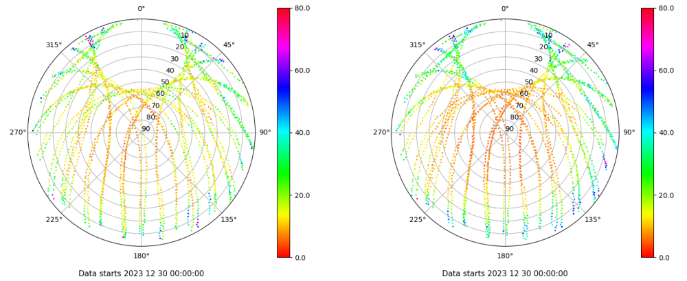
Skyplot for station PENI. Parameter M1C Data file PENI00ESP_R_2023364.xtr Skyplot for station PENI. Parameter M2P Data file PENI00ESP_R_2023364.xtr
