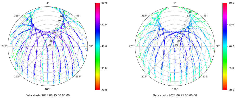
Skyplot for station PENI. Signal to Noise S1C Data file PENI00ESP_R_2023176.xtr Skyplot for station PENI. Signal to Noise S2P Data file PENI00ESP_R_2023176.xtr
