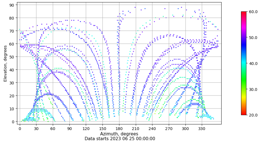
Azimuth-elevation plot for station PENI. Signal to Noise S1C Data file PENI00ESP_R_2023176.xtr
