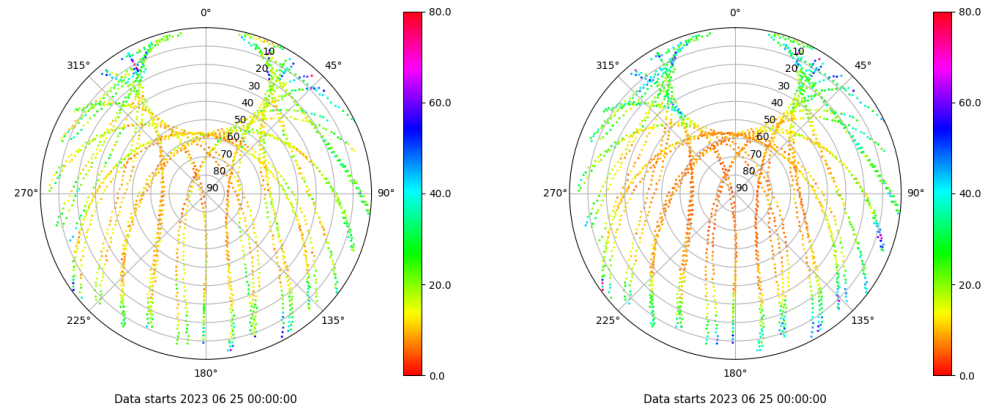
Skyplot for station PENI. Parameter M1C Data file PENI00ESP_R_2023176.xtr Skyplot for station PENI. Parameter M2P Data file PENI00ESP_R_2023176.xtr
