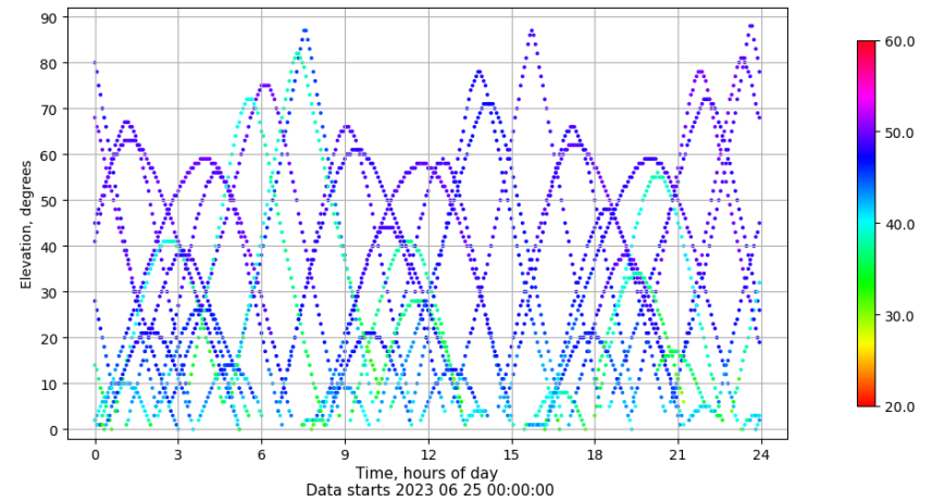
Time-elevation plot for station PENI. Signal to Noise S1C Data file PENI00ESP_R_2023176.xtr
