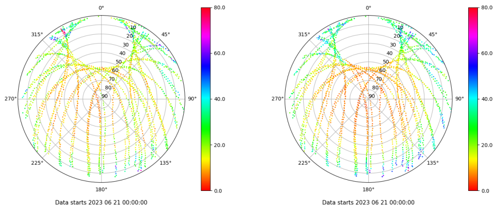
Skyplot for station PENI. Parameter M1C Data file PENI00ESP_R_2023172.xtr Skyplot for station PENI. Parameter M2P Data file PENI00ESP_R_2023172.xtr
