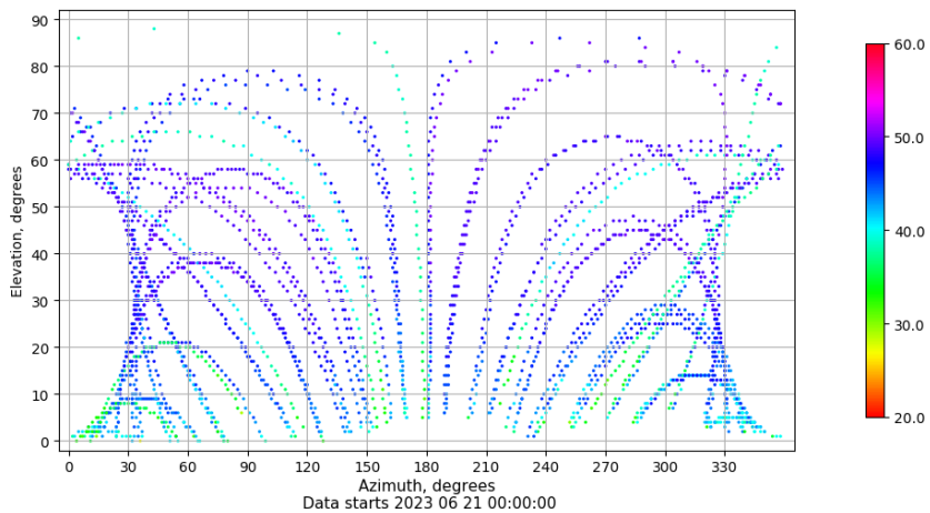
Azimuth-elevation plot for station PENI. Signal to Noise S1C Data file PENI00ESP_R_2023172.xtr
