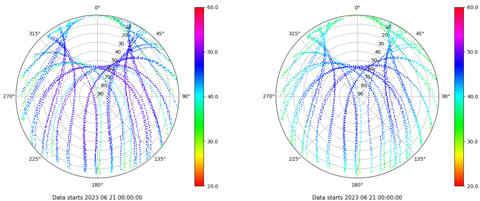
Skyplot for station PENI. Signal to Noise S1C Data file PENI00ESP_R_2023172.xtr Skyplot for station PENI. Signal to Noise S2P Data file PENI00ESP_R_2023172.xtr
