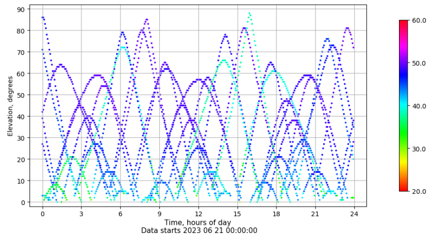
Time-elevation plot for station PENI. Signal to Noise S1C Data file PENI00ESP_R_2023172.xtr
