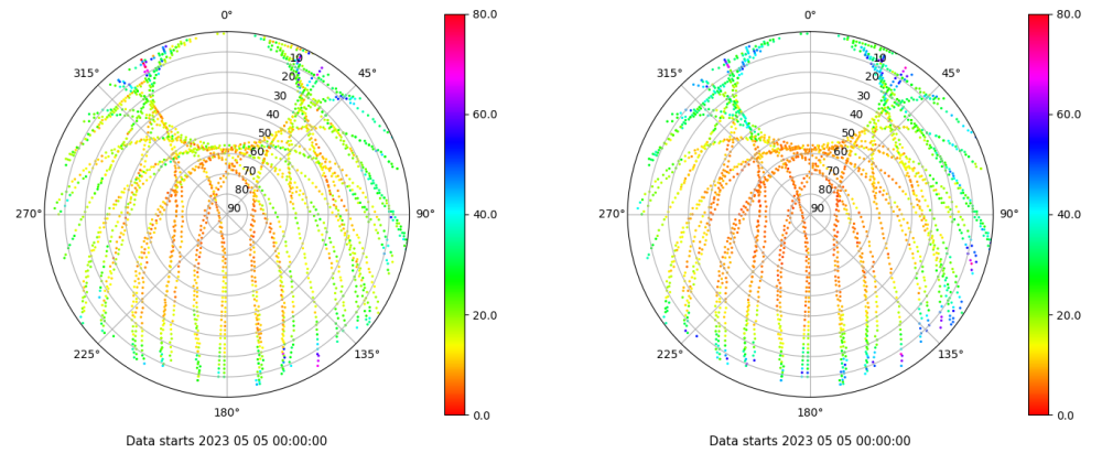
Skyplot for station PENI. Parameter M1C Data file PENI00ESP_R_2023125.xtr Skyplot for station PENI. Parameter M2P Data file PENI00ESP_R_2023125.xtr
