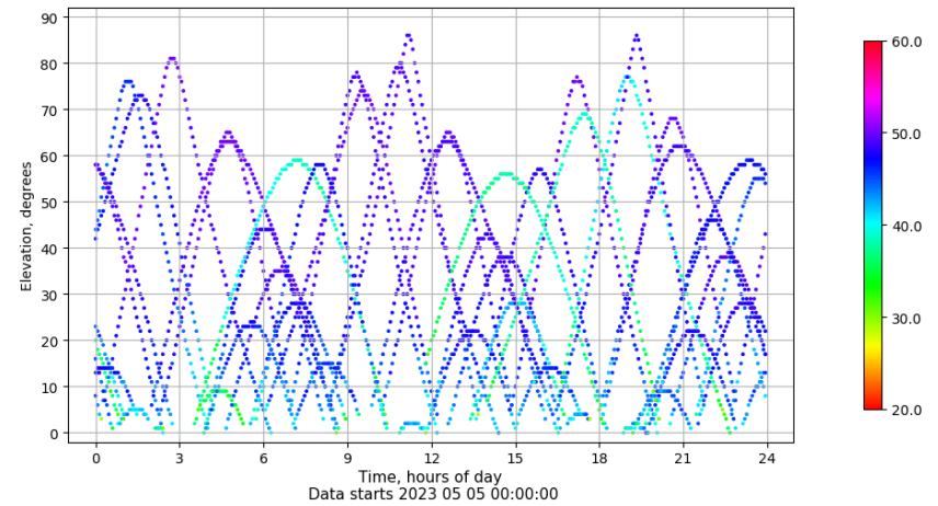
Time-elevation plot for station PENI. Signal to Noise S1C Data file PENI00ESP_R_2023125.xtr
