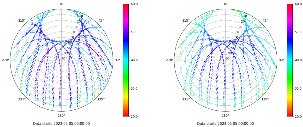
Skyplot for station PENI. Signal to Noise S1C Data file PENI00ESP_R_2023125.xtr Skyplot for station PENI. Signal to Noise S2P Data file PENI00ESP_R_2023125.xtr
