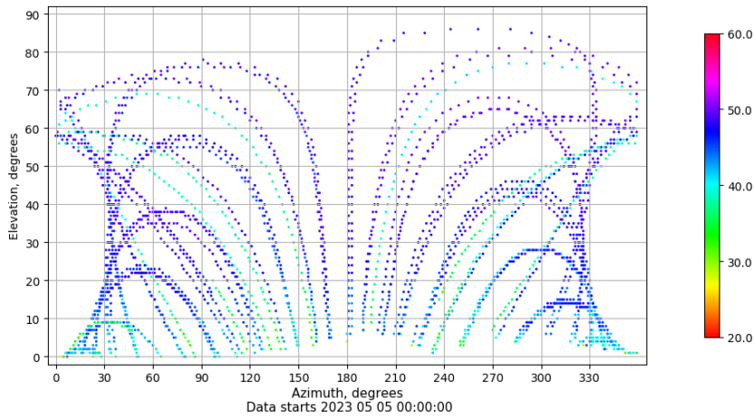
Azimuth-elevation plot for station PENI. Signal to Noise S1C Data file PENI00ESP_R_2023125.xtr
