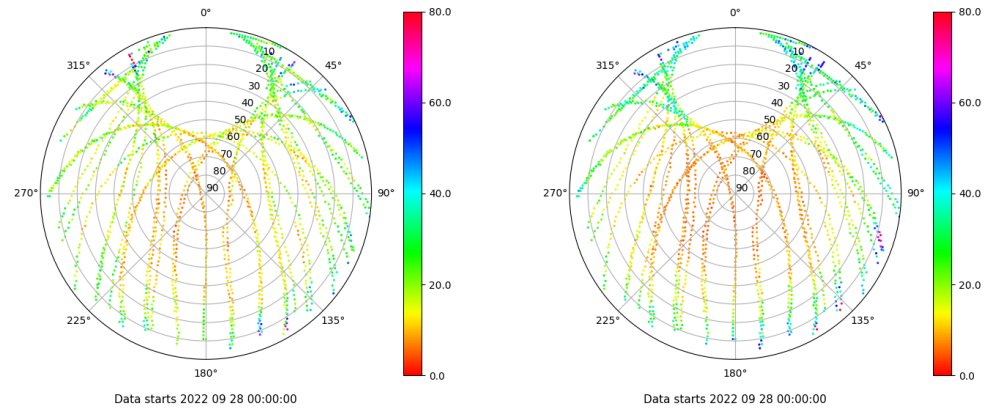
Skyplot for station PENI. Parameter M1C Data file PENI00ESP_R_2022271.xtr Skyplot for station PENI. Parameter M2P Data file PENI00ESP_R_2022271.xtr
