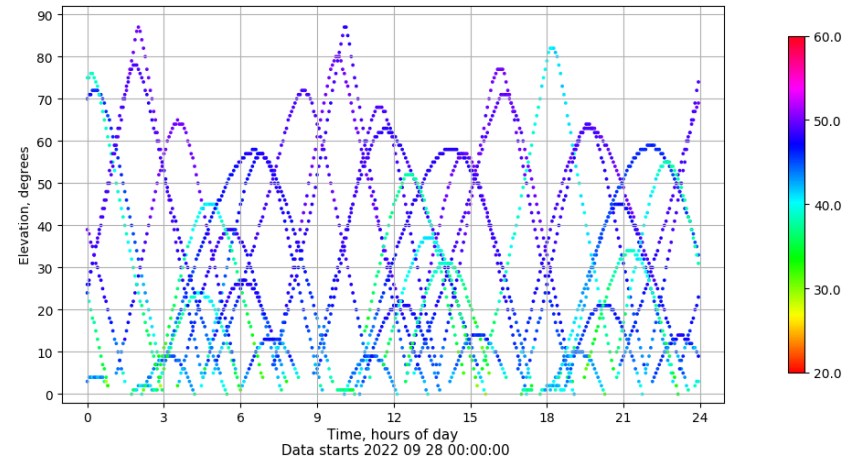
Time-elevation plot for station PENI. Signal to Noise S1C Data file PENI00ESP_R_2022271.xtr
