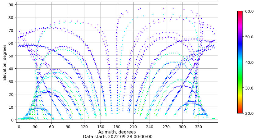
Azimuth-elevation plot for station PENI. Signal to Noise S1C Data file PENI00ESP_R_2022271.xtr
