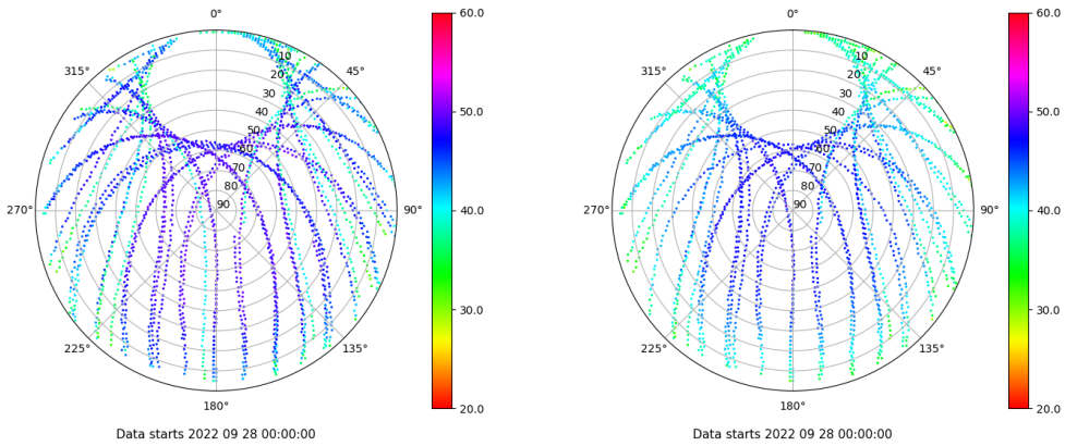
Skyplot for station PENI. Signal to Noise S1C Data file PENI00ESP_R_2022271.xtr Skyplot for station PENI. Signal to Noise S2P Data file PENI00ESP_R_2022271.xtr
