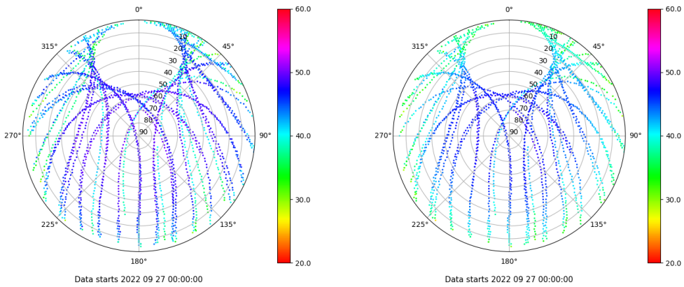
Skyplot for station PENI. Signal to Noise S1C Data file PENI00ESP_R_2022270.xtr Skyplot for station PENI. Signal to Noise S2P Data file PENI00ESP_R_2022270.xtr
