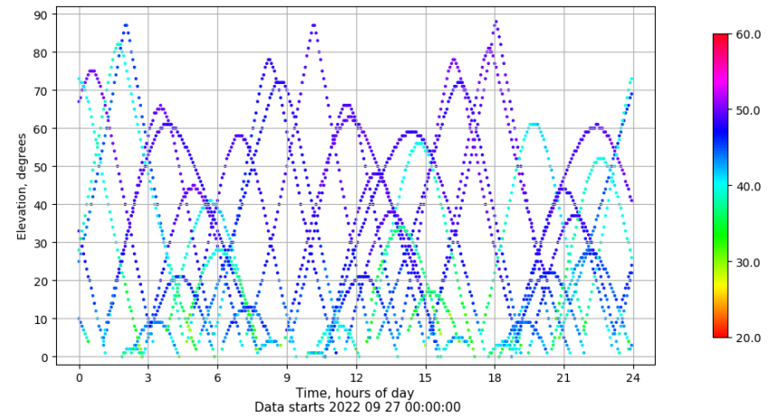
Time-elevation plot for station PENI. Signal to Noise S1C Data file PENI00ESP_R_2022270.xtr
