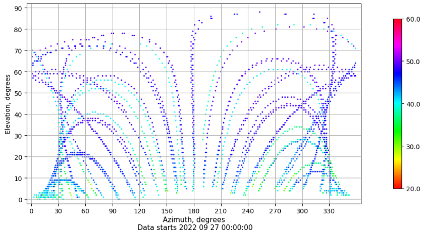
Azimuth-elevation plot for station PENI. Signal to Noise S1C Data file PENI00ESP_R_2022270.xtr
