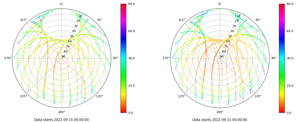
Skyplot for station PENI. Parameter M1C Data file PENI00ESP_R_2022258.xtr Skyplot for station PENI. Parameter M2P Data file PENI00ESP_R_2022258.xtr
