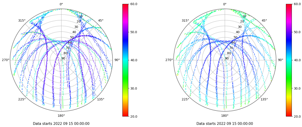
Skyplot for station PENI. Signal to Noise S1C Data file PENI00ESP_R_2022258.xtr Skyplot for station PENI. Signal to Noise S2P Data file PENI00ESP_R_2022258.xtr
