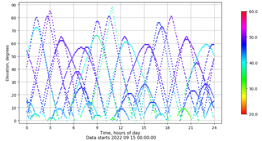
Time-elevation plot for station PENI. Signal to Noise S1C Data file PENI00ESP_R_2022258.xtr
