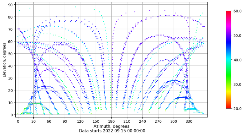
Azimuth-elevation plot for station PENI. Signal to Noise S1C Data file PENI00ESP_R_2022258.xtr
