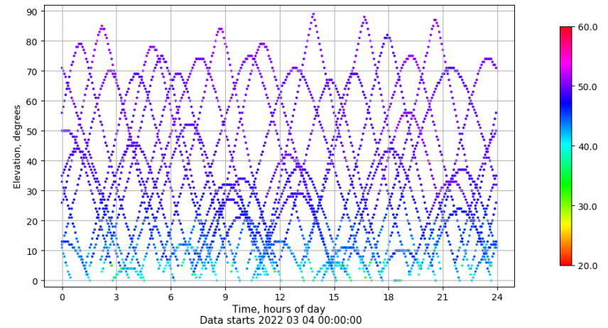
Time-elevation plot for station PENI. Signal to Noise S1C Data file PENI00ESP_R_2022063.xtr
