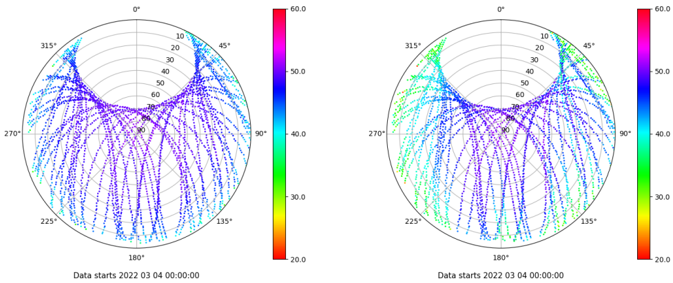
Skyplot for station PENI. Signal to Noise S1C Data file PENI00ESP_R_2022063.xtr Skyplot for station PENI. Signal to Noise S2W Data file PENI00ESP_R_2022063.xtr
