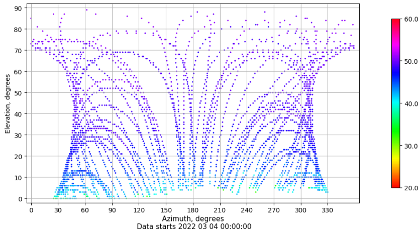
Azimuth-elevation plot for station PENI. Signal to Noise S1C Data file PENI00ESP_R_2022063.xtr
