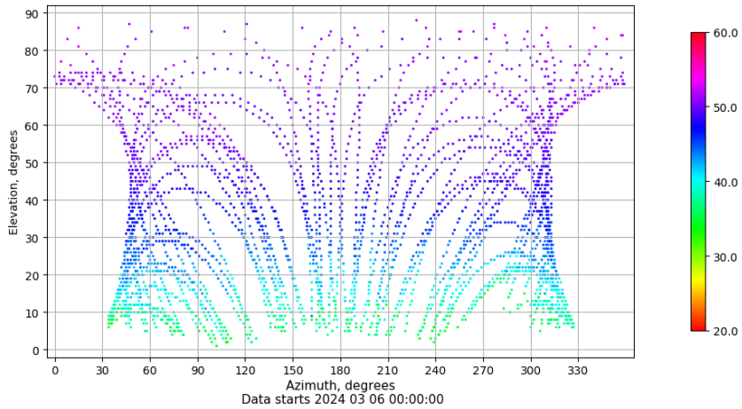
Azimuth-elevation plot for station MOLI. Signal to Noise S1C Data file MOLI00ESP_R_2024066.xtr
