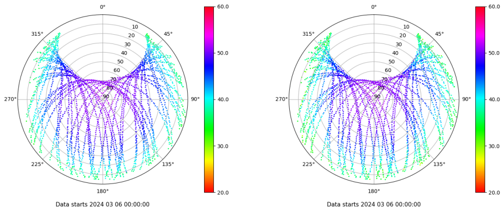
Skyplot for station MOLI. Signal to Noise S1C Data file MOLI00ESP_R_2024066.xtr Skyplot for station MOLI. Signal to Noise S2W Data file MOLI00ESP_R_2024066.xtr
