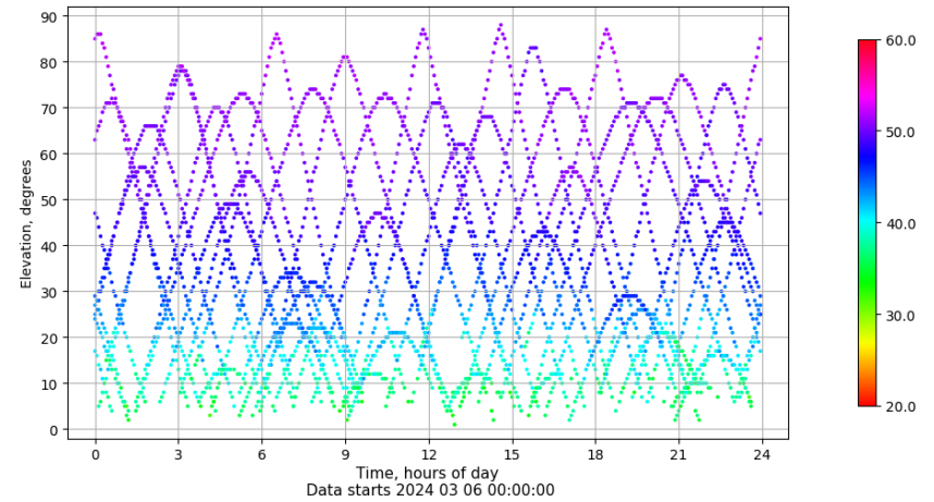
Time-elevation plot for station MOLI. Signal to Noise S1C Data file MOLI00ESP_R_2024066.xtr
