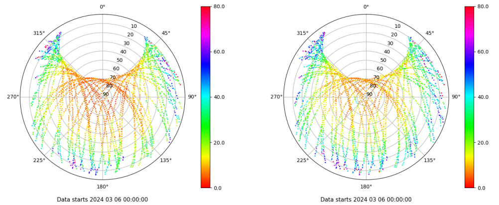
Skyplot for station MOLI. Parameter M1C Data file MOLI00ESP_R_2024066.xtr Skyplot for station MOLI. Parameter M2W Data file MOLI00ESP_R_2024066.xtr
