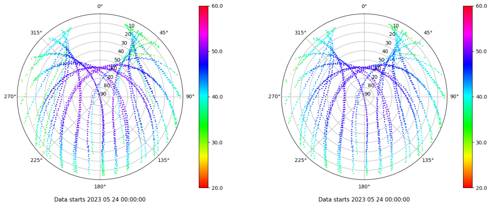
Skyplot for station MOLI. Signal to Noise S1C Data file MOLI00ESP_R_2023144.xtr Skyplot for station MOLI. Signal to Noise S2P Data file MOLI00ESP_R_2023144.xtr
