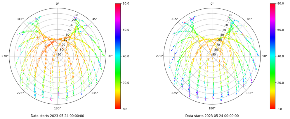
Skyplot for station MOLI. Parameter M1C Data file MOLI00ESP_R_2023144.xtr Skyplot for station MOLI. Parameter M2P Data file MOLI00ESP_R_2023144.xtr
