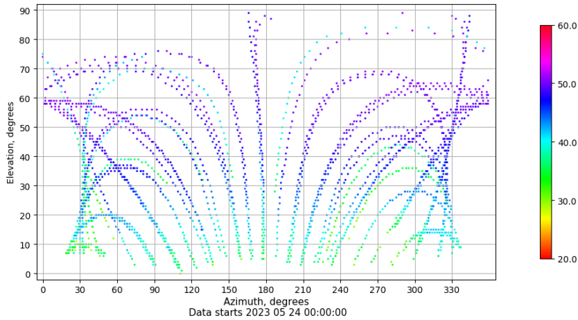
Azimuth-elevation plot for station MOLI. Signal to Noise S1C Data file MOLI00ESP_R_2023144.xtr
