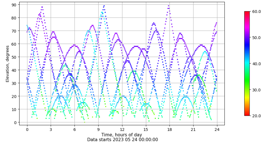
Time-elevation plot for station MOLI. Signal to Noise S1C Data file MOLI00ESP_R_2023144.xtr
