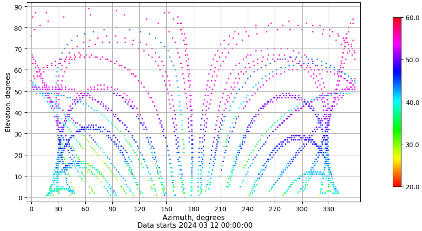
Azimuth-elevation plot for station MLLL. Signal to Noise S1C Data file MLLL00ESP_R_2024072.xtr
