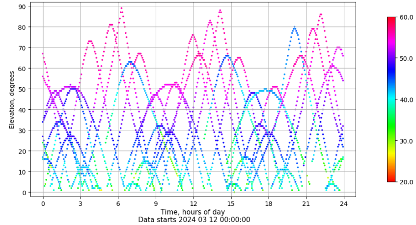
Time-elevation plot for station MLLL. Signal to Noise S1C Data file MLLL00ESP_R_2024072.xtr
