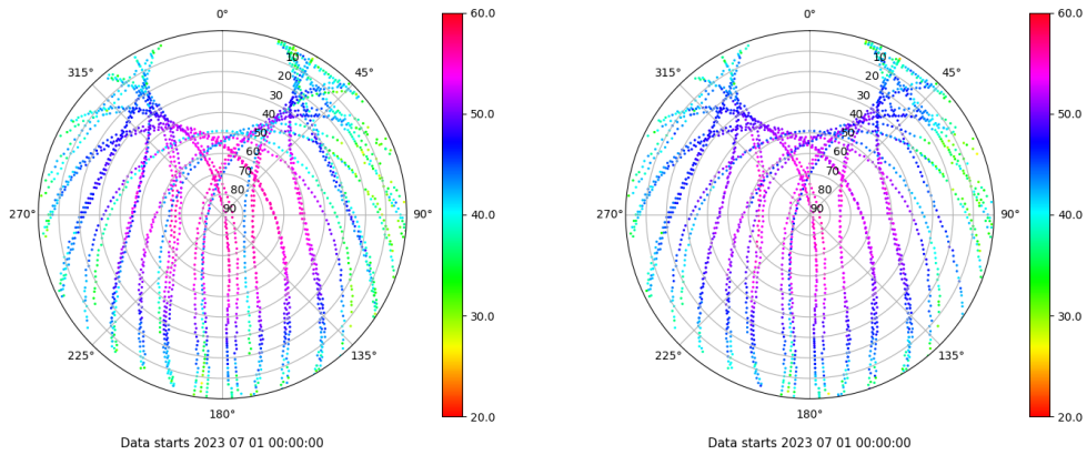
Skyplot for station MLLL. Signal to Noise S1C Data file MLLL00ESP_R_2023182.xtr Skyplot for station MLLL. Signal to Noise S2C Data file MLLL00ESP_R_2023182.xtr
