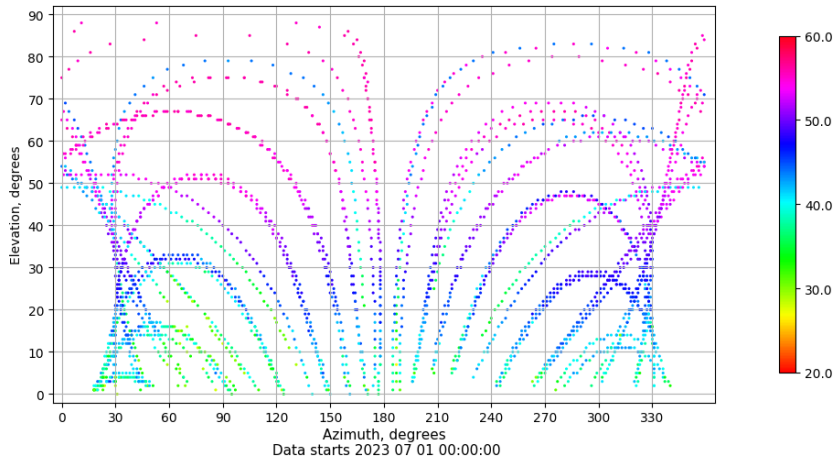
Azimuth-elevation plot for station MLLL. Signal to Noise S1C Data file MLLL00ESP_R_2023182.xtr
