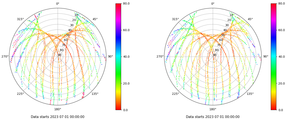
Skyplot for station MLLL. Parameter M1C Data file MLLL00ESP_R_2023182.xtr Skyplot for station MLLL. Parameter M2C Data file MLLL00ESP_R_2023182.xtr
