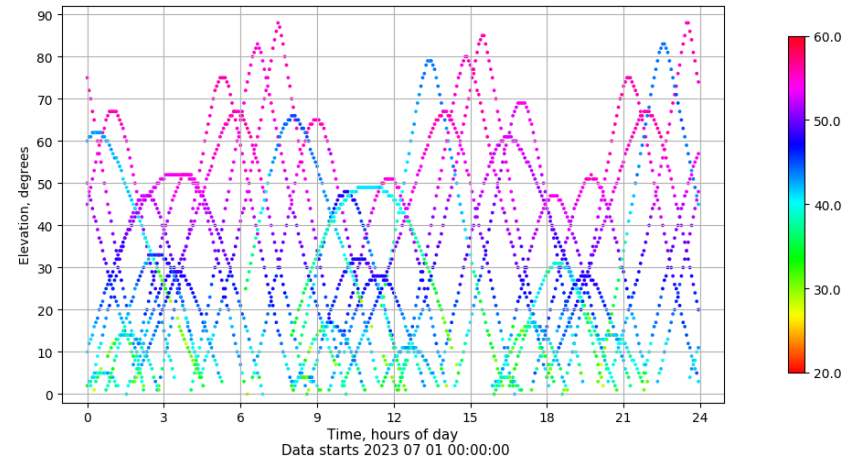
Time-elevation plot for station MLLL. Signal to Noise S1C Data file MLLL00ESP_R_2023182.xtr
