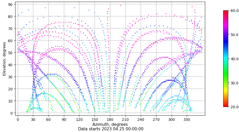
Azimuth-elevation plot for station MLLL. Signal to Noise S1C Data file MLLL00ESP_R_2023115.xtr
