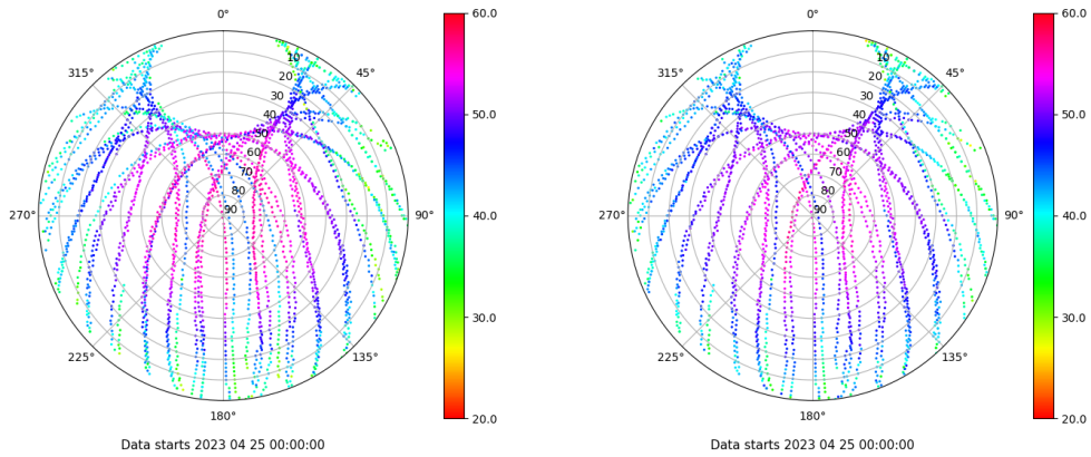
Skyplot for station MLLL. Signal to Noise S1C Data file MLLL00ESP_R_2023115.xtr Skyplot for station MLLL. Signal to Noise S2C Data file MLLL00ESP_R_2023115.xtr
