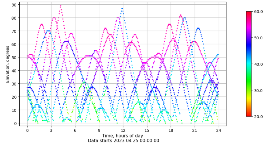
Time-elevation plot for station MLLL. Signal to Noise S1C Data file MLLL00ESP_R_2023115.xtr
