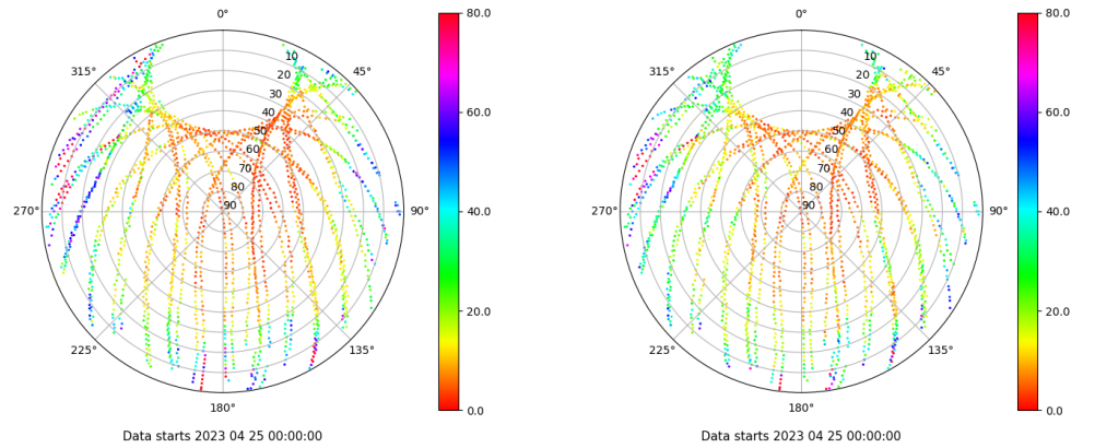
Skyplot for station MLLL. Parameter M1C Data file MLLL00ESP_R_2023115.xtr Skyplot for station MLLL. Parameter M2C Data file MLLL00ESP_R_2023115.xtr
