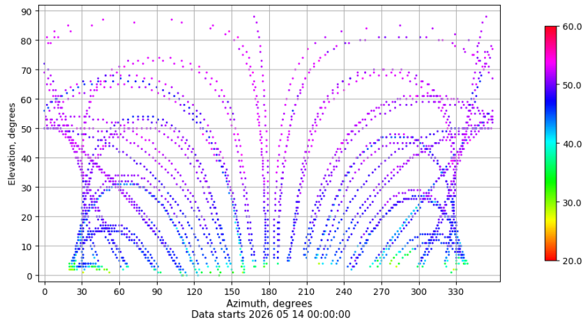
Azimuth-elevation plot for station MELI. Signal to Noise S1C Data file MELI00ESP_R_2026134.xtr
