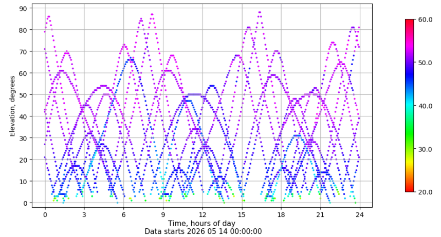
Time-elevation plot for station MELI. Signal to Noise S1C Data file MELI00ESP_R_2026134.xtr
