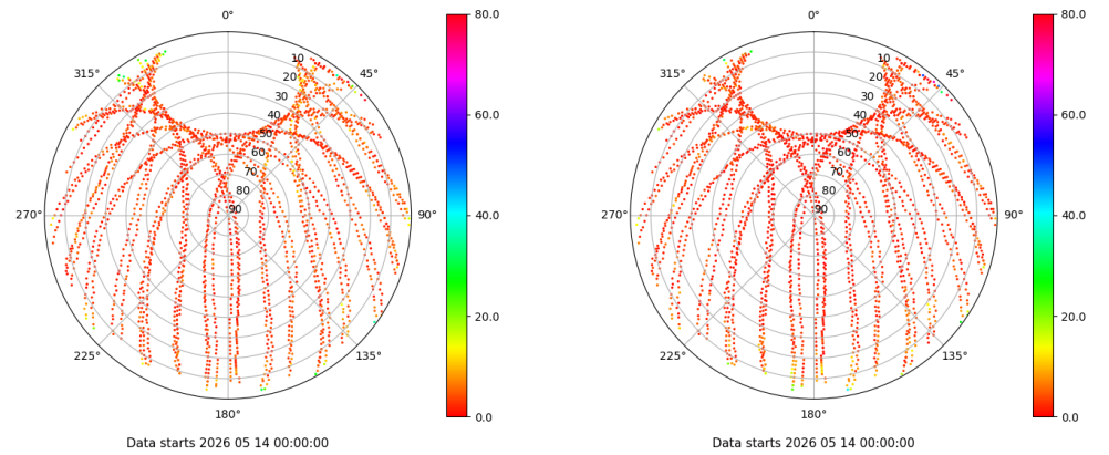
Skyplot for station MELI. Parameter M1C Data file MELI00ESP_R_2026134.xtr Skyplot for station MELI. Parameter M2C Data file MELI00ESP_R_2026134.xtr
