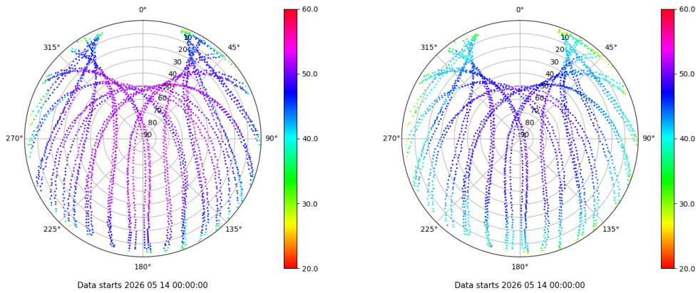
Skyplot for station MELI. Signal to Noise S1C Data file MELI00ESP_R_2026134.xtr Skyplot for station MELI. Signal to Noise S2C Data file MELI00ESP_R_2026134.xtr
