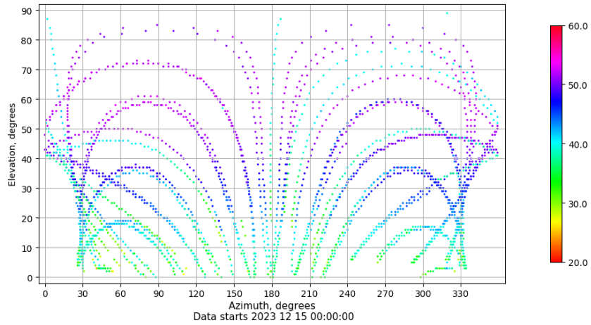
Azimuth-elevation plot for station MASP. Signal to Noise S1C Data file MASP00ESP_R_2023349.xtr
