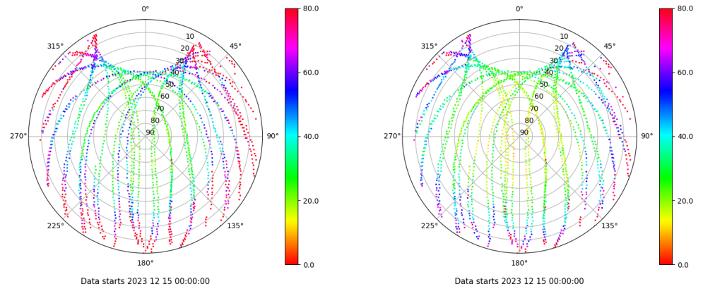
Skyplot for station MASP. Parameter M1C Data file MASP00ESP_R_2023349.xtr Skyplot for station MASP. Parameter M2C Data file MASP00ESP_R_2023349.xtr
