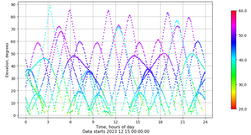
Time-elevation plot for station MASP. Signal to Noise S1C Data file MASP00ESP_R_2023349.xtr
