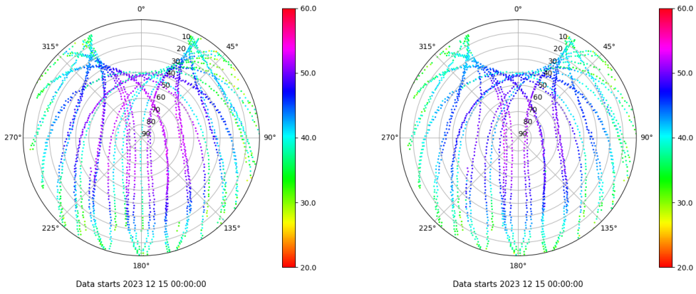
Skyplot for station MASP. Signal to Noise S1C Data file MASP00ESP_R_2023349.xtr Skyplot for station MASP. Signal to Noise S2C Data file MASP00ESP_R_2023349.xtr
