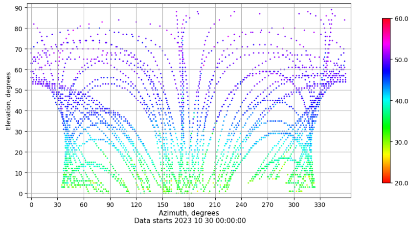
Azimuth-elevation plot for station MASP. Signal to Noise S1C Data file MASP00ESP_R_2023303.xtr
