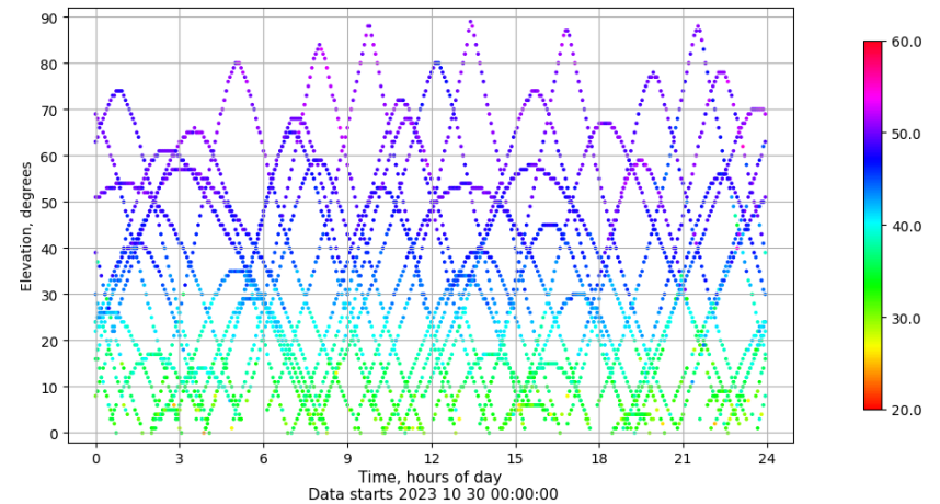
Time-elevation plot for station MASP. Signal to Noise S1C Data file MASP00ESP_R_2023303.xtr
