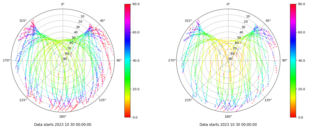
Skyplot for station MASP. Parameter M1C Data file MASP00ESP_R_2023303.xtr Skyplot for station MASP. Parameter M2L Data file MASP00ESP_R_2023303.xtr
