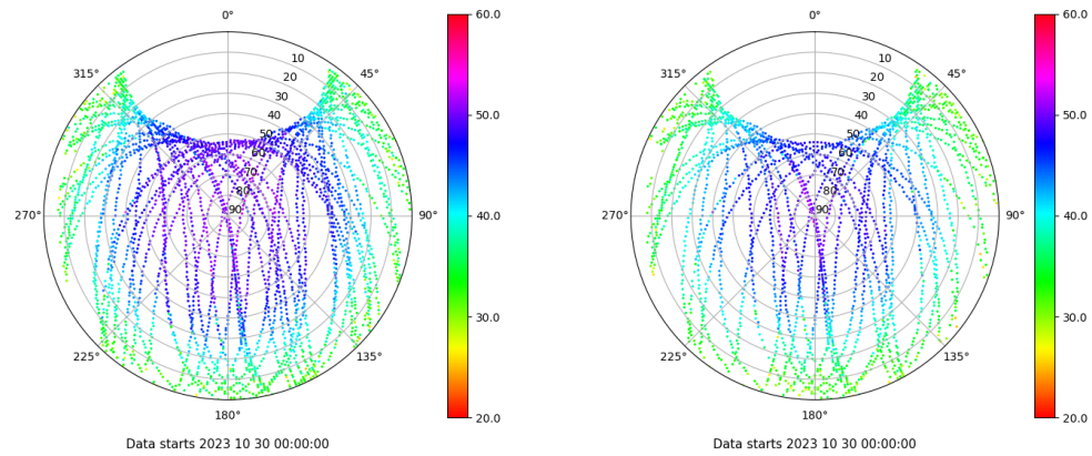
Skyplot for station MASP. Signal to Noise S1C Data file MASP00ESP_R_2023303.xtr Skyplot for station MASP. Signal to Noise S2L Data file MASP00ESP_R_2023303.xtr
