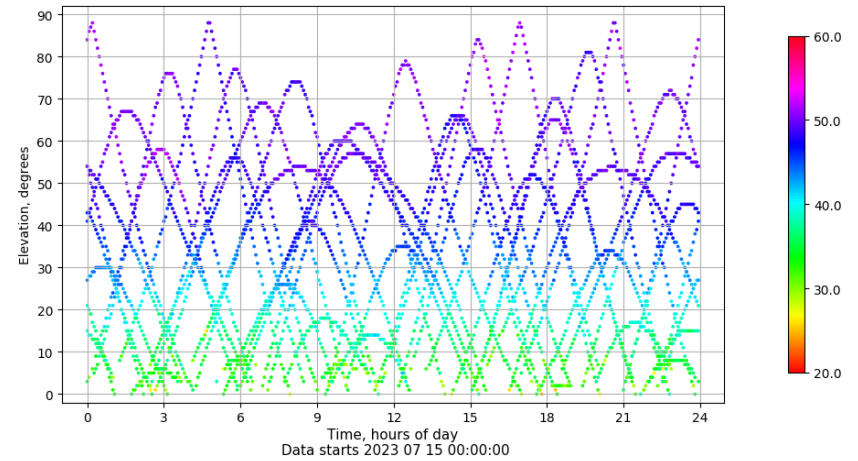
Time-elevation plot for station MASP. Signal to Noise S1C Data file MASP00ESP_R_2023196.xtr
