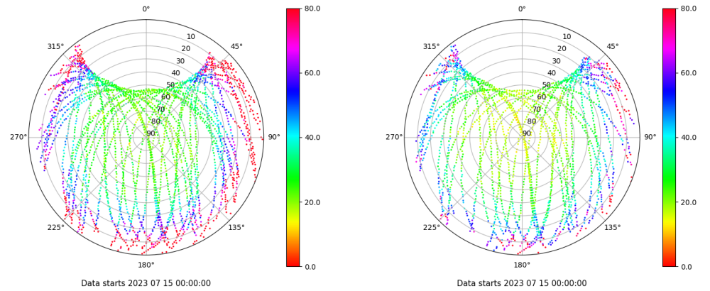
Skyplot for station MASP. Parameter M1C Data file MASP00ESP_R_2023196.xtr Skyplot for station MASP. Parameter M2L Data file MASP00ESP_R_2023196.xtr
