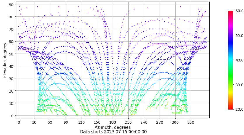
Azimuth-elevation plot for station MASP. Signal to Noise S1C Data file MASP00ESP_R_2023196.xtr
