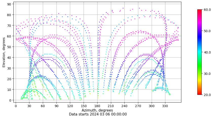
Azimuth-elevation plot for station MALL. Signal to Noise S1C Data file MALL00ESP_R_2024066.xtr
