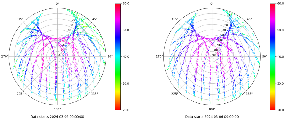
Skyplot for station MALL. Signal to Noise S1C Data file MALL00ESP_R_2024066.xtr Skyplot for station MALL. Signal to Noise S2C Data file MALL00ESP_R_2024066.xtr
