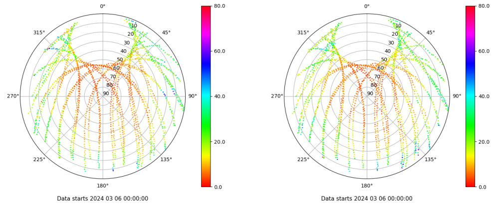
Skyplot for station MALL. Parameter M1C Data file MALL00ESP_R_2024066.xtr Skyplot for station MALL. Parameter M2C Data file MALL00ESP_R_2024066.xtr
