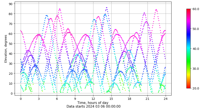
Time-elevation plot for station MALL. Signal to Noise S1C Data file MALL00ESP_R_2024066.xtr
