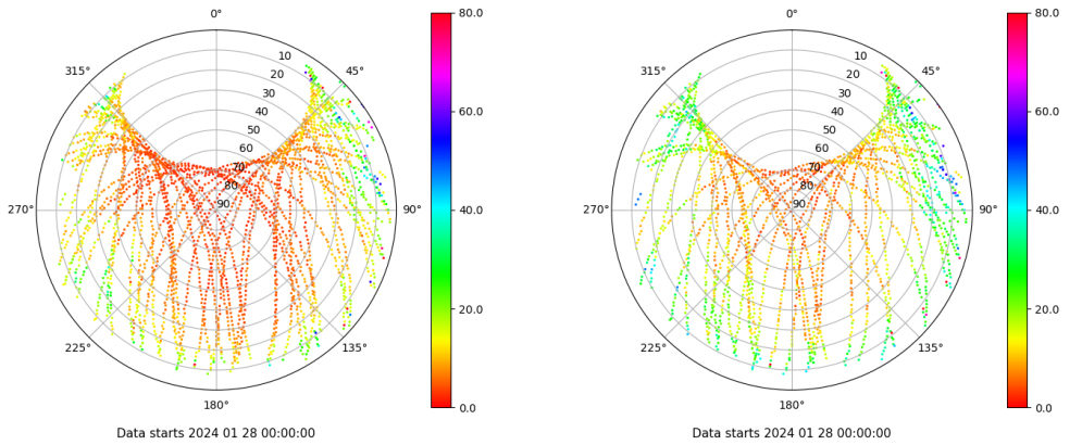
Skyplot for station MALL. Parameter M1C Data file MALL00ESP_R_2024028.xtr Skyplot for station MALL. Parameter M2S Data file MALL00ESP_R_2024028.xtr
