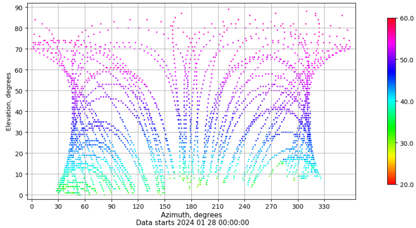
Azimuth-elevation plot for station MALL. Signal to Noise S1C Data file MALL00ESP_R_2024028.xtr
