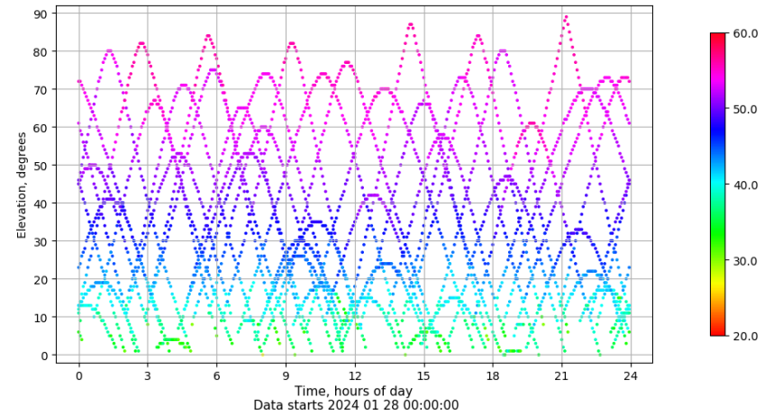
Time-elevation plot for station MALL. Signal to Noise S1C Data file MALL00ESP_R_2024028.xtr
