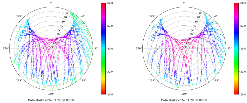
Skyplot for station MALL. Signal to Noise S1C Data file MALL00ESP_R_2024028.xtr Skyplot for station MALL. Signal to Noise S2S Data file MALL00ESP_R_2024028.xtr
