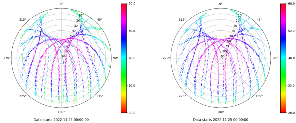
Skyplot for station MALL. Signal to Noise S1C Data file MALL00ESP_R_2022329.xtr Skyplot for station MALL. Signal to Noise S2C Data file MALL00ESP_R_2022329.xtr
