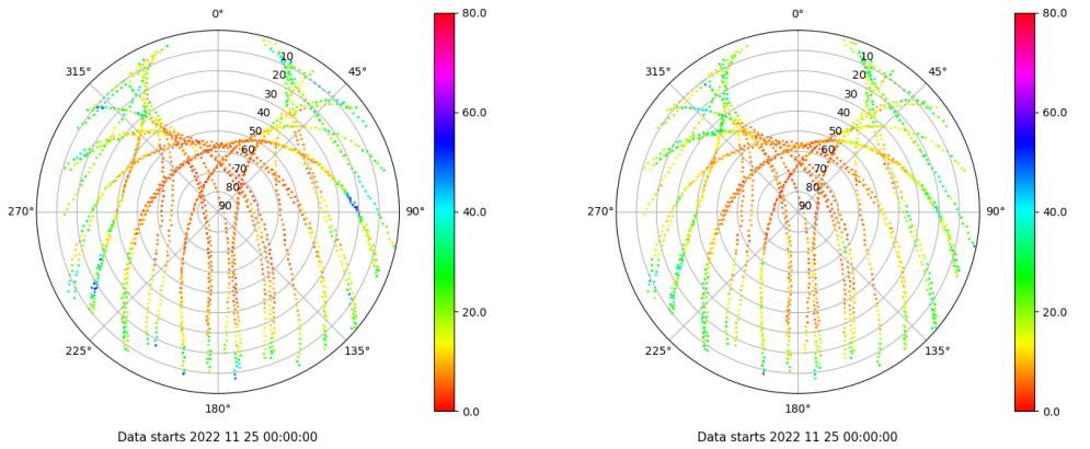
Skyplot for station MALL. Parameter M1C Data file MALL00ESP_R_2022329.xtr Skyplot for station MALL. Parameter M2C Data file MALL00ESP_R_2022329.xtr
