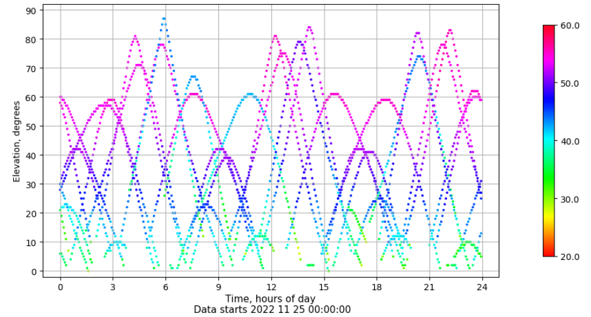
Time-elevation plot for station MALL. Signal to Noise S1C Data file MALL00ESP_R_2022329.xtr
