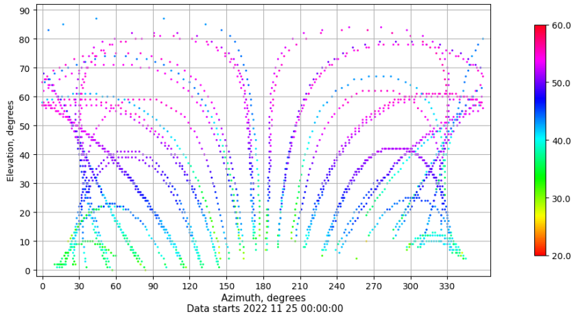
Azimuth-elevation plot for station MALL. Signal to Noise S1C Data file MALL00ESP_R_2022329.xtr
