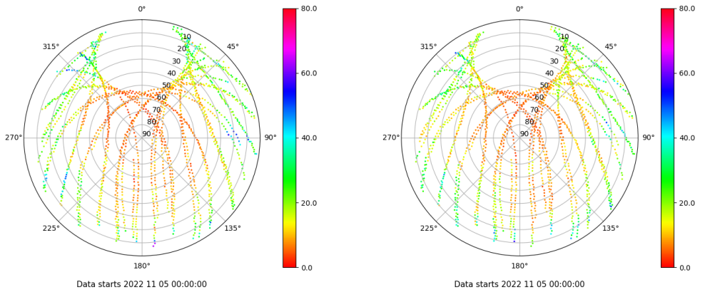
Skyplot for station MALL. Parameter M1C Data file MALL00ESP_R_2022309.xtr Skyplot for station MALL. Parameter M2C Data file MALL00ESP_R_2022309.xtr
