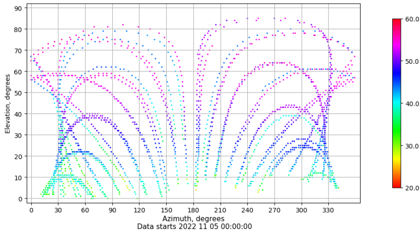
Azimuth-elevation plot for station MALL. Signal to Noise S1C Data file MALL00ESP_R_2022309.xtr
