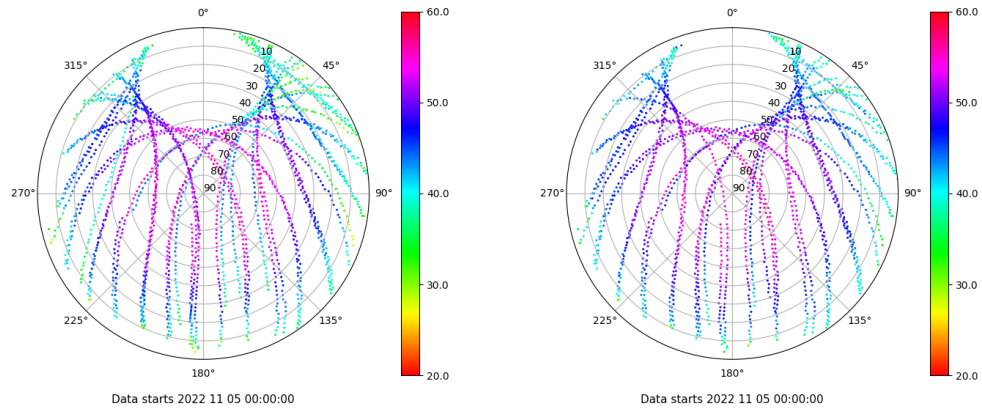
Skyplot for station MALL. Signal to Noise S1C Data file MALL00ESP_R_2022309.xtr Skyplot for station MALL. Signal to Noise S2C Data file MALL00ESP_R_2022309.xtr
