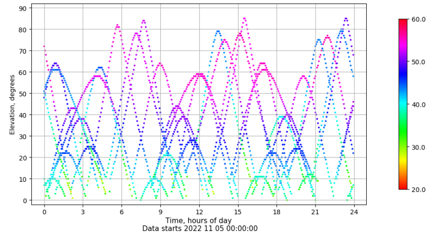
Time-elevation plot for station MALL. Signal to Noise S1C Data file MALL00ESP_R_2022309.xtr
