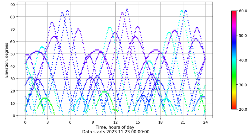
Time-elevation plot for station MALA. Signal to Noise S1C Data file MALA00ESP_R_2023327.xtr
