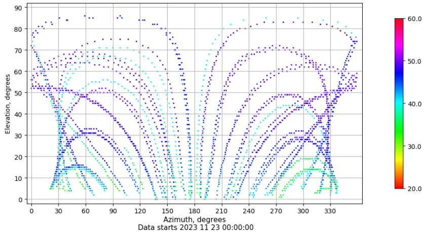
Azimuth-elevation plot for station MALA. Signal to Noise S1C Data file MALA00ESP_R_2023327.xtr
