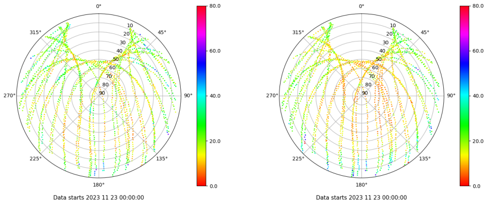
Skyplot for station MALA. Parameter M1C Data file MALA00ESP_R_2023327.xtr Skyplot for station MALA. Parameter M2P Data file MALA00ESP_R_2023327.xtr
