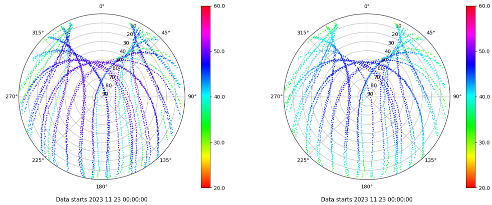
Skyplot for station MALA. Signal to Noise S1C Data file MALA00ESP_R_2023327.xtr Skyplot for station MALA. Signal to Noise S2P Data file MALA00ESP_R_2023327.xtr
