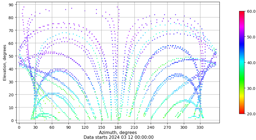
Azimuth-elevation plot for station LZ02. Signal to Noise S1C Data file LZ0200ESP_R_2024072.xtr
