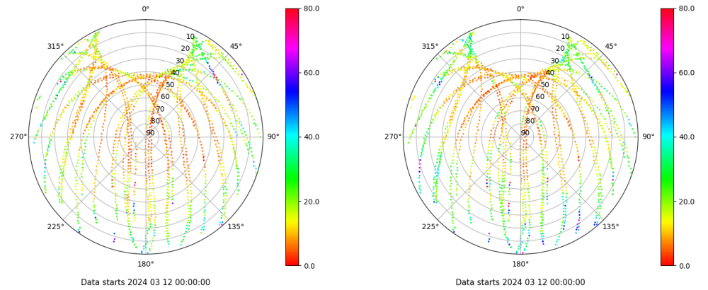
Skyplot for station LZ02. Parameter M1C Data file LZ0200ESP_R_2024072.xtr Skyplot for station LZ02. Parameter M2P Data file LZ0200ESP_R_2024072.xtr
