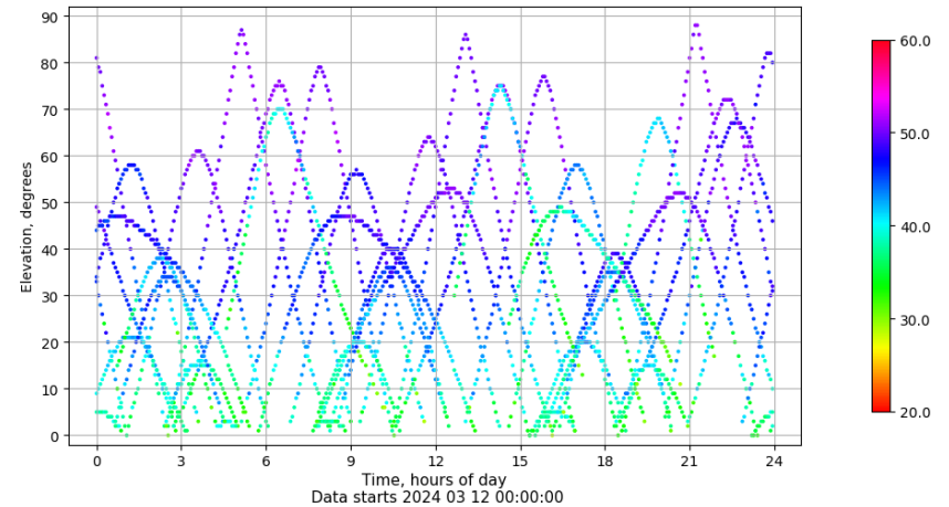
Time-elevation plot for station LZ02. Signal to Noise S1C Data file LZ0200ESP_R_2024072.xtr
