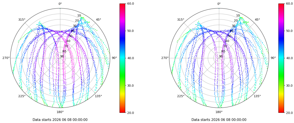
Skyplot for station LRES. Signal to Noise S1C Data file LRES00ESP_R_2026159.xtr Skyplot for station LRES. Signal to Noise S2P Data file LRES00ESP_R_2026159.xtr
