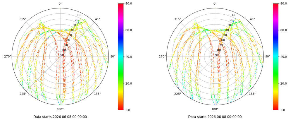
Skyplot for station LRES. Parameter M1C Data file LRES00ESP_R_2026159.xtr Skyplot for station LRES. Parameter M2P Data file LRES00ESP_R_2026159.xtr
