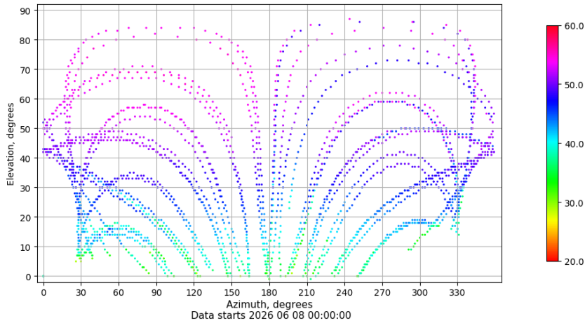
Azimuth-elevation plot for station LRES. Signal to Noise S1C Data file LRES00ESP_R_2026159.xtr
