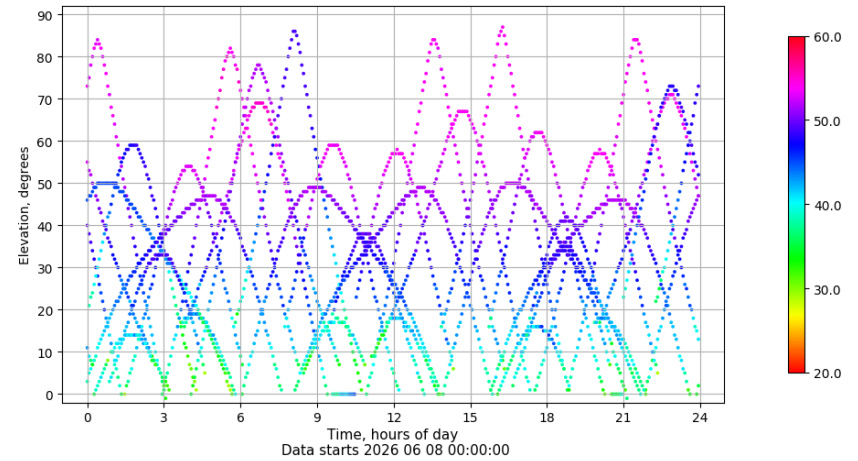
Time-elevation plot for station LRES. Signal to Noise S1C Data file LRES00ESP_R_2026159.xtr
