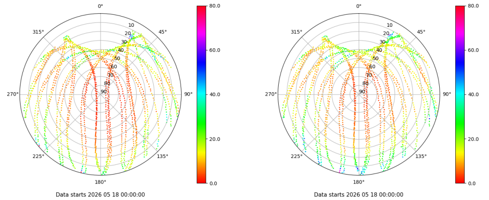
Skyplot for station LRES. Parameter M1C Data file LRES00ESP_R_2026138.xtr Skyplot for station LRES. Parameter M2P Data file LRES00ESP_R_2026138.xtr
