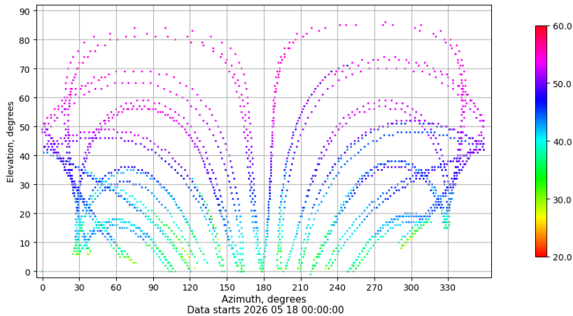
Azimuth-elevation plot for station LRES. Signal to Noise S1C Data file LRES00ESP_R_2026138.xtr
