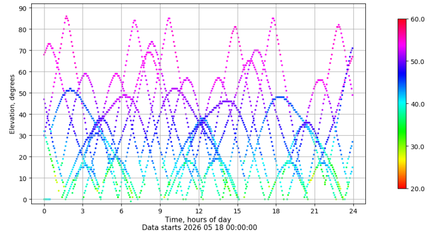
Time-elevation plot for station LRES. Signal to Noise S1C Data file LRES00ESP_R_2026138.xtr
