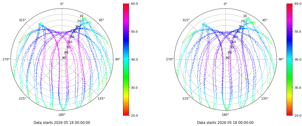
Skyplot for station LRES. Signal to Noise S1C Data file LRES00ESP_R_2026138.xtr Skyplot for station LRES. Signal to Noise S2P Data file LRES00ESP_R_2026138.xtr
