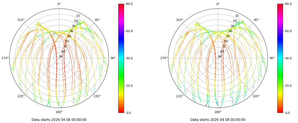
Skyplot for station LRES. Parameter M1C Data file LRES00ESP_R_2026098.xtr Skyplot for station LRES. Parameter M2P Data file LRES00ESP_R_2026098.xtr
