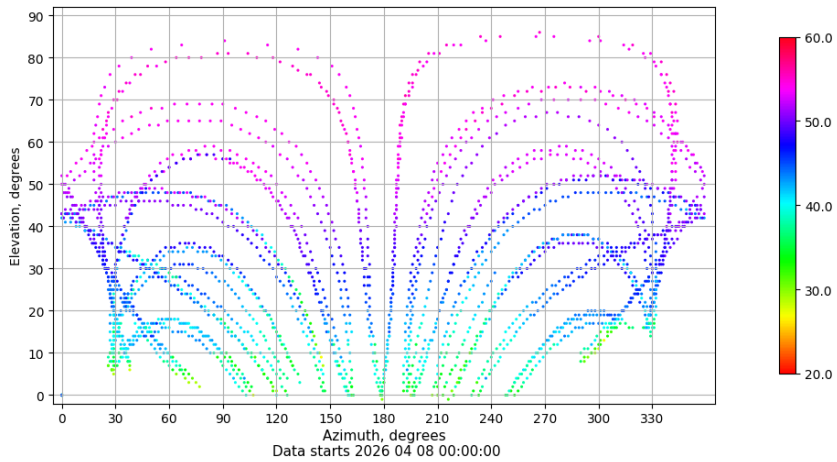
Azimuth-elevation plot for station LRES. Signal to Noise S1C Data file LRES00ESP_R_2026098.xtr
