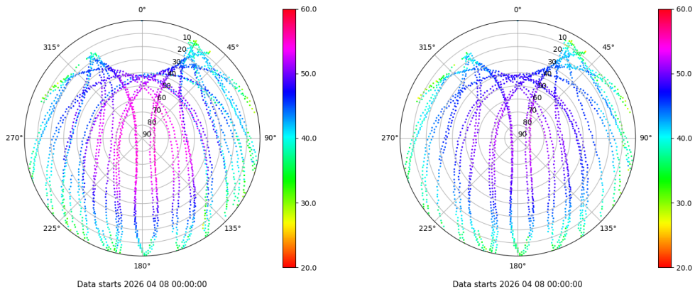
Skyplot for station LRES. Signal to Noise S1C Data file LRES00ESP_R_2026098.xtr Skyplot for station LRES. Signal to Noise S2P Data file LRES00ESP_R_2026098.xtr
