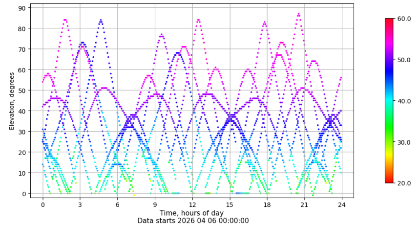
Time-elevation plot for station LRES. Signal to Noise S1C Data file LRES00ESP_R_2026096.xtr
