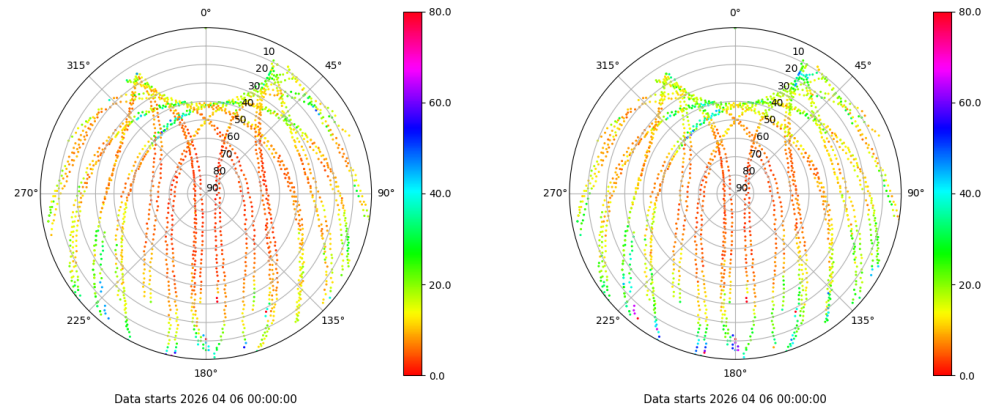
Skyplot for station LRES. Parameter M1C Data file LRES00ESP_R_2026096.xtr Skyplot for station LRES. Parameter M2P Data file LRES00ESP_R_2026096.xtr
