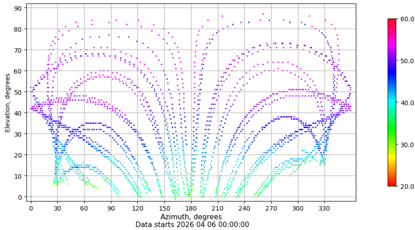
Azimuth-elevation plot for station LRES. Signal to Noise S1C Data file LRES00ESP_R_2026096.xtr
