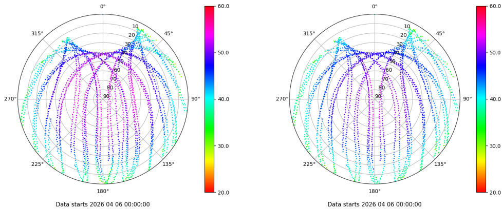
Skyplot for station LRES. Signal to Noise S1C Data file LRES00ESP_R_2026096.xtr Skyplot for station LRES. Signal to Noise S2P Data file LRES00ESP_R_2026096.xtr
