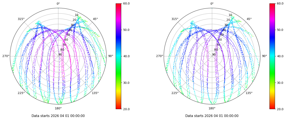
Skyplot for station LRES. Signal to Noise S1C Data file LRES00ESP_R_2026091.xtr Skyplot for station LRES. Signal to Noise S2P Data file LRES00ESP_R_2026091.xtr
