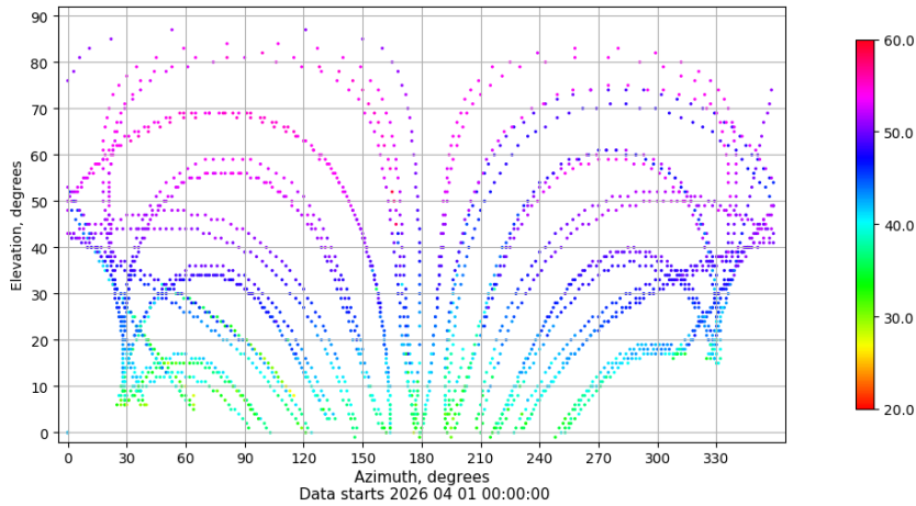
Azimuth-elevation plot for station LRES. Signal to Noise S1C Data file LRES00ESP_R_2026091.xtr
