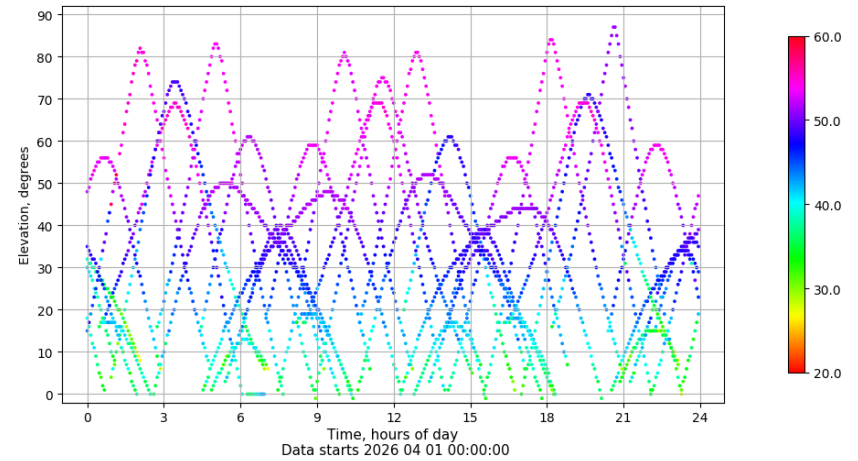
Time-elevation plot for station LRES. Signal to Noise S1C Data file LRES00ESP_R_2026091.xtr
