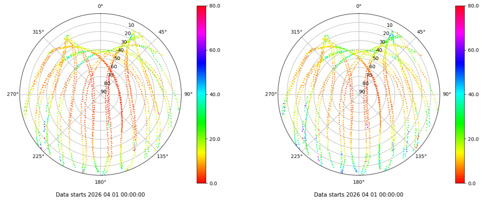
Skyplot for station LRES. Parameter M1C Data file LRES00ESP_R_2026091.xtr Skyplot for station LRES. Parameter M2P Data file LRES00ESP_R_2026091.xtr
